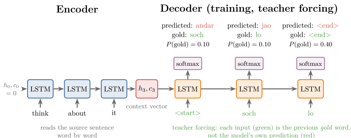
Figure 4: Training on one observation. The decoder’s input at each step (green) is the previous gold word, not the model’s own prediction (red)
