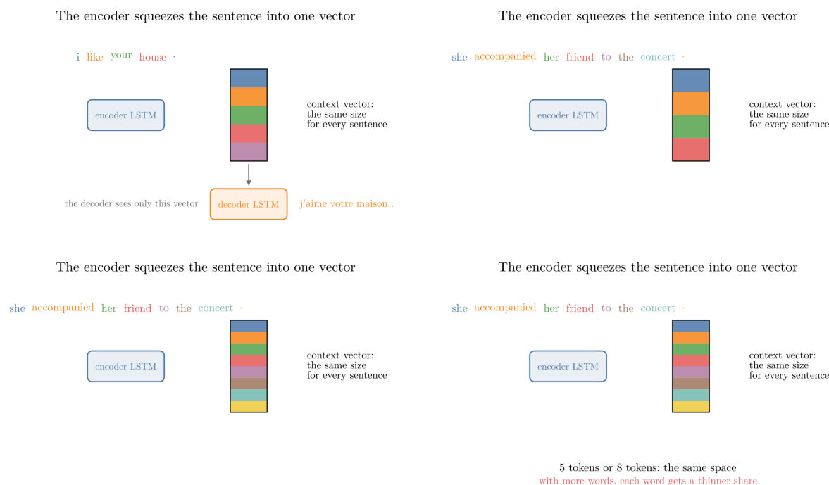
Figure 3: The encoder reads one word per step and ends with one context vector of fixed size, the decoder’s only view of the input. A 5-token sentence and an 8-token sentence end in the same space, so each word gets a thinner share. A picture of the idea, not of the LSTM’s actual numbers
