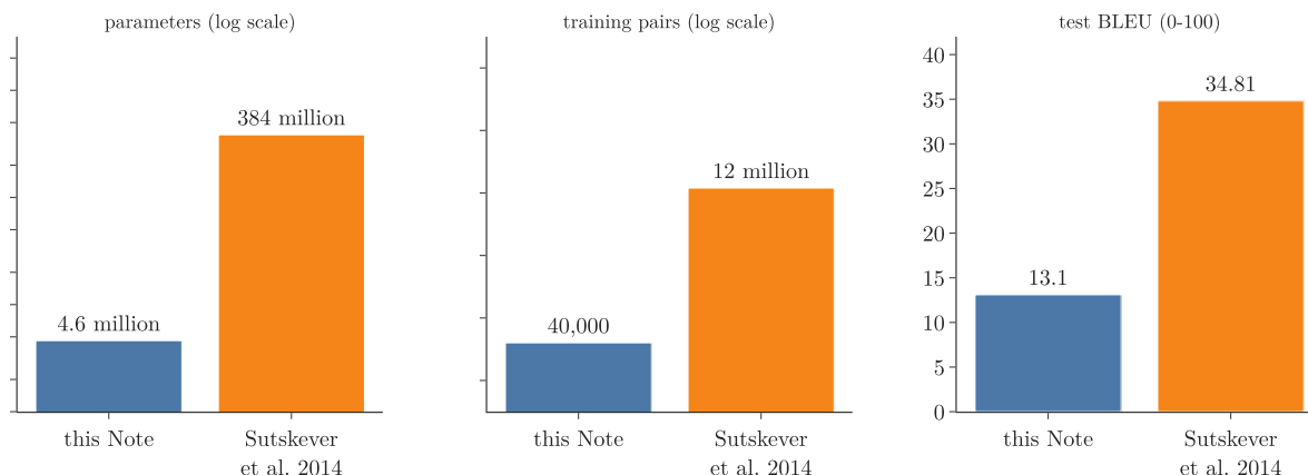
Figure 9: The Notebook’s model against the original model of Sutskever et al. (2014): parameters and training pairs (log scales), and test BLEU
