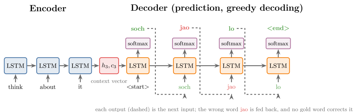
Figure 6: Prediction with greedy decoding on the toy example. Each output becomes the next input (dashed). The wrong word “jao” at step 2 is fed back into step 3, and no gold word corrects it
