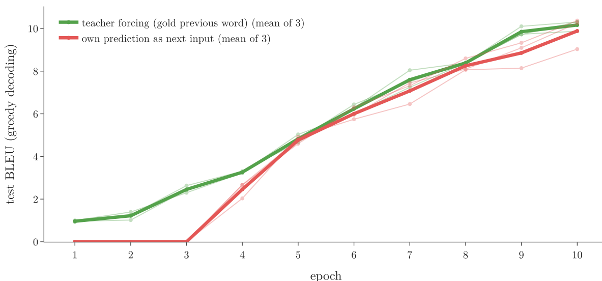
Figure 7: Test BLEU after each epoch. Thin lines: 3 runs each; thick lines: their mean. With teacher forcing (green) the model starts scoring at once; trained on its own predictions (red) it scores 0 for 3 epochs
