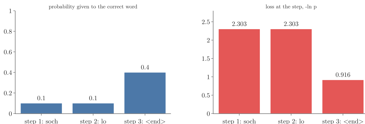
Figure 5: The worked example. Left: the probability the decoder gave each correct word. Right: the loss at each step, -\ln p . A probability of 0.1 costs 2.303, one of 0.4 costs 0.916; the mean, 1.84, is what Keras reports
