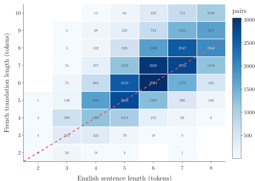
Figure 2: The 40,000 English–French training pairs of section 6 (English up to 8 tokens, French up to 10, punctuation counted), counted by the length of each side. Only 30% of the pairs lie on the dashed diagonal, where both sides have the same length
