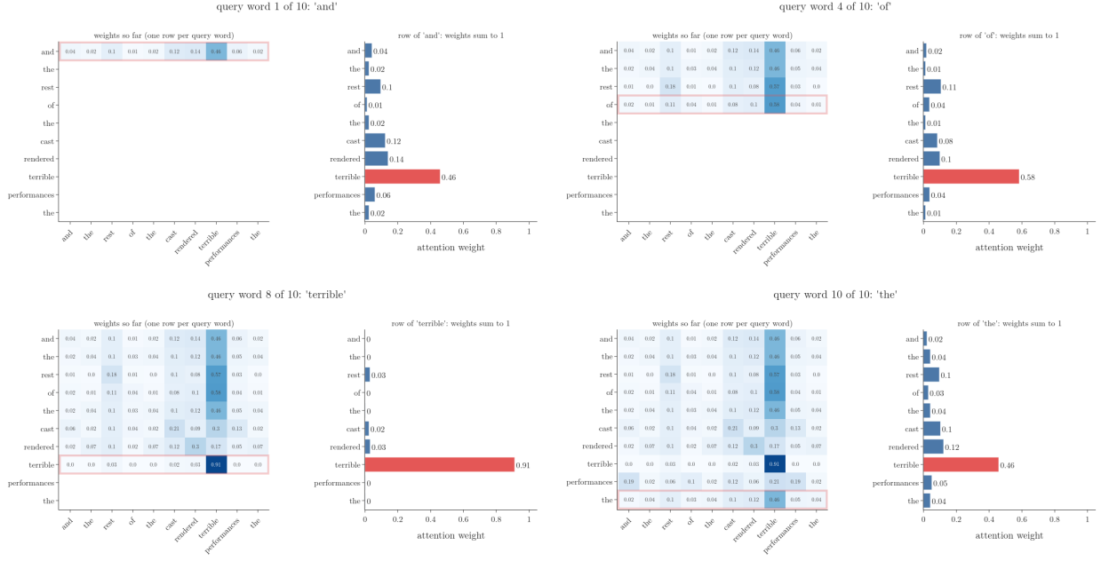
Figure 10: The learned weights forming one query word at a time. Left: the weight matrix filling row by row. Right: the current query word's weights, which sum to 1; the largest is red
