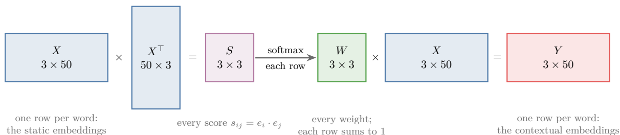
Figure 4: The whole sentence at once, for “money bank grows”. One product gives every score, a softmax on each row gives every weight, and a second product gives every contextual embedding
