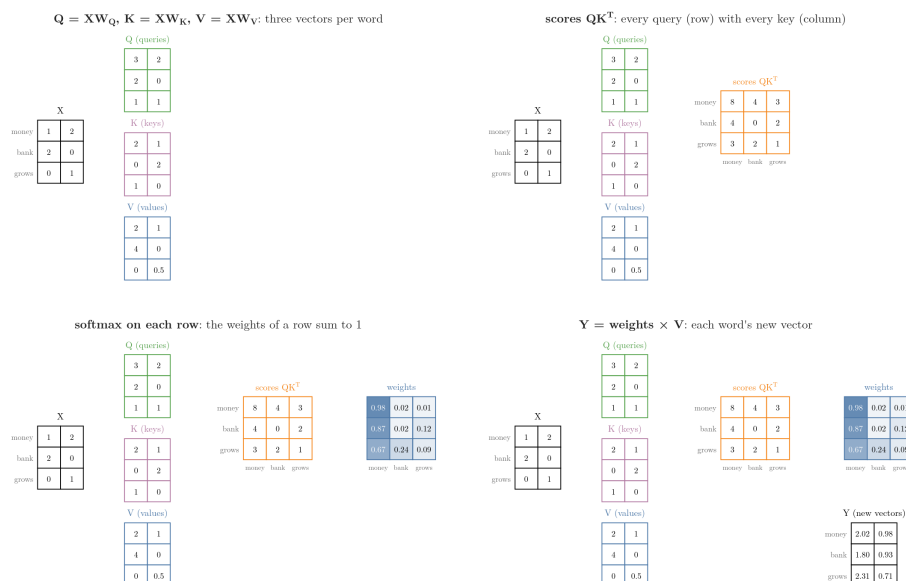
Figure 8: The worked example, one operation per frame: X ; then Q , K , V ; the scores QK^T ; the weights after a softmax on each row (darker = larger); and Y , the weights times V (a full numeric walk-through after StatQuest, “The matrix math behind transformer neural networks, one step at a time!!!”; the numbers are our own)
