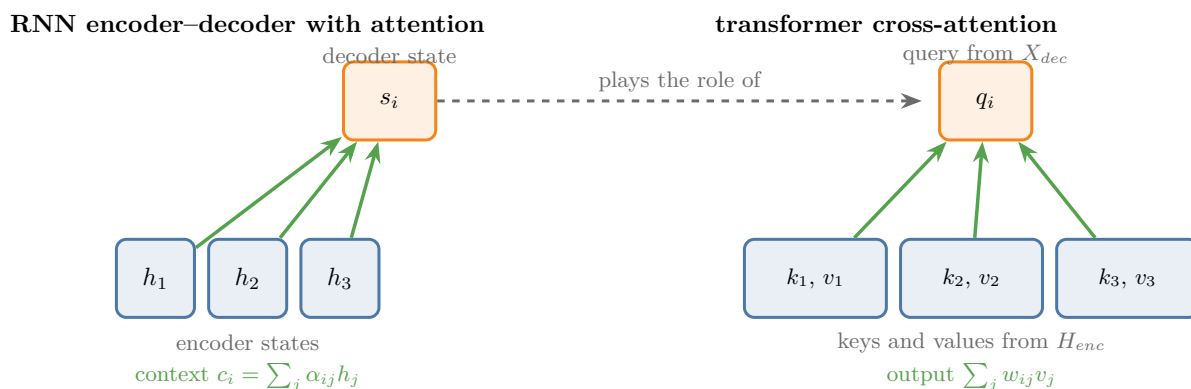
Figure 6: Left: in the RNN encoder–decoder, the decoder state s_i weighs the encoder states h_j to build its context vector. Right: in cross-attention, the query q_i from the decoder weighs the keys from the encoder and mixes the values
