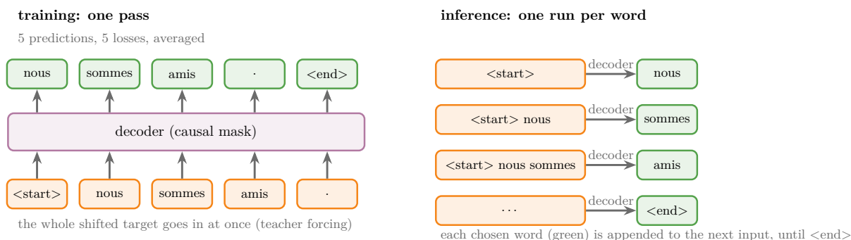
Figure 5: Left: in training, the whole shifted target goes into the decoder at once and all five positions are predicted in one pass. Right: in inference, the decoder runs once per new word, and each chosen word is appended to the next input
