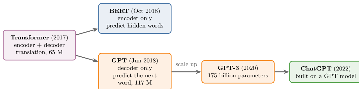
Figure 13: From the 2017 transformer to ChatGPT: the encoder alone became BERT, the decoder alone became GPT, and scaling GPT up led to GPT-3 and ChatGPT
