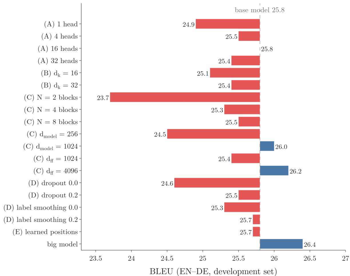
Figure 11: Table 3 as bars around the base model’s 25.8 BLEU: blue rows beat the base model, red rows fall below it
