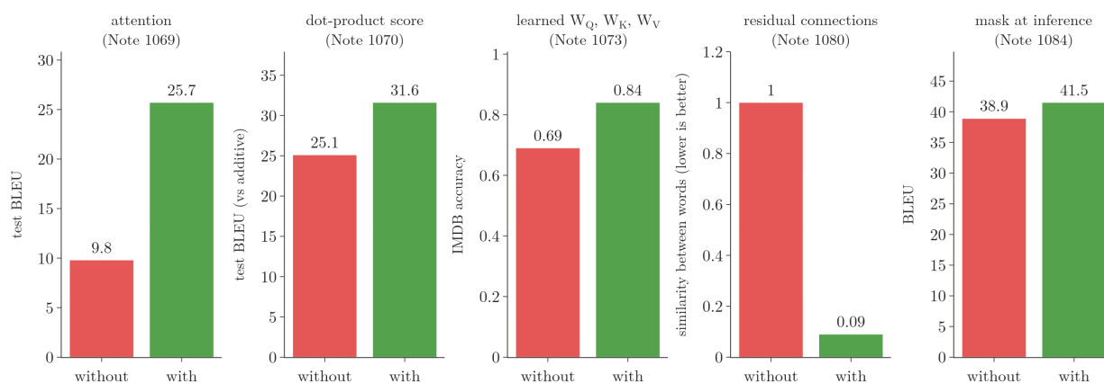
Figure 6: Five parts of the transformer and the effect measured in the Note that teaches each one: the metric without the part (red) and with it (green). For the residual connections, the metric is the similarity between words after one block, where lower is better
