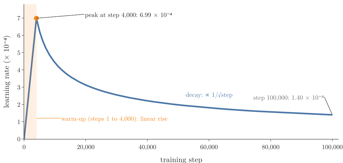
Figure 7: The learning rate of the base model over its 100,000 training steps
