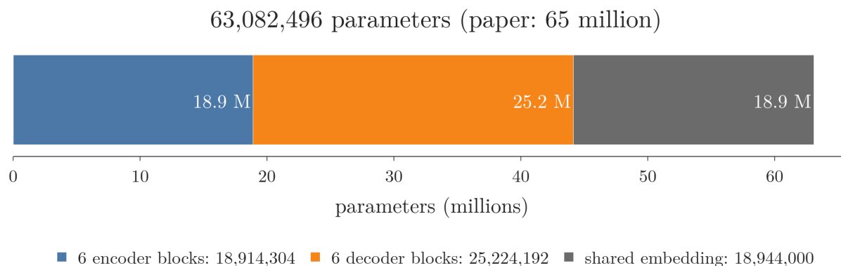
Figure 4: Where the base model’s 63,082,496 parameters sit: the 6 encoder blocks, the 6 decoder blocks and the shared embedding
