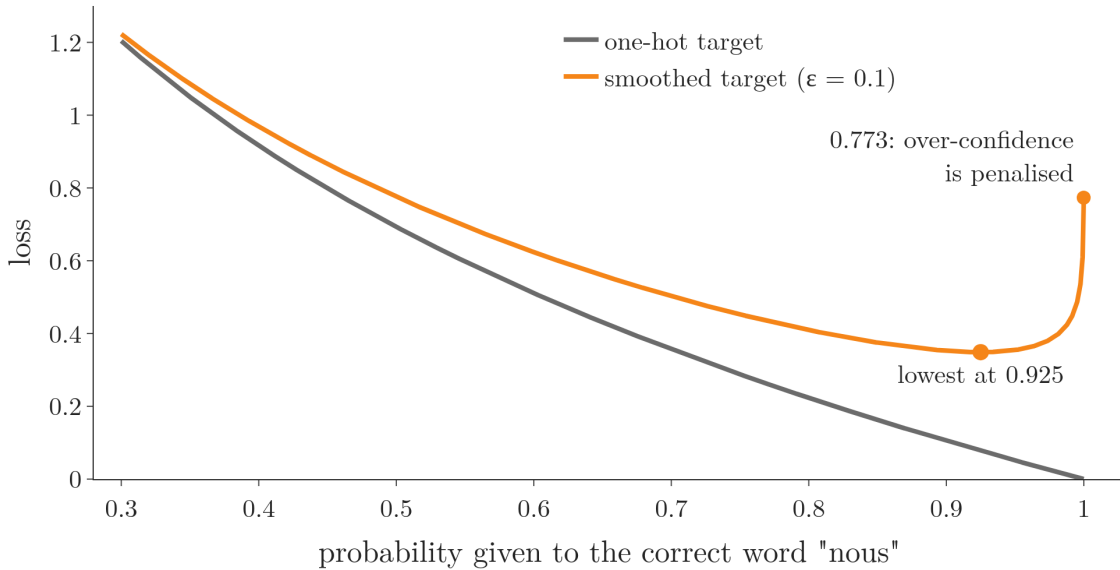
Figure 9: The two losses as the probability of the correct word “nous” grows from 0.30 to 0.9999, with the rest shared evenly. The one-hot loss keeps falling towards certainty; the smoothed loss is lowest at 0.925 and rises again
