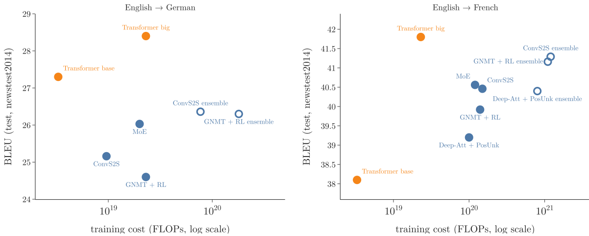
Figure 10: Table 2 of the paper: BLEU against training cost. Orange: the transformer. Hollow circles: ensembles. ByteNet has no listed cost and is left out
