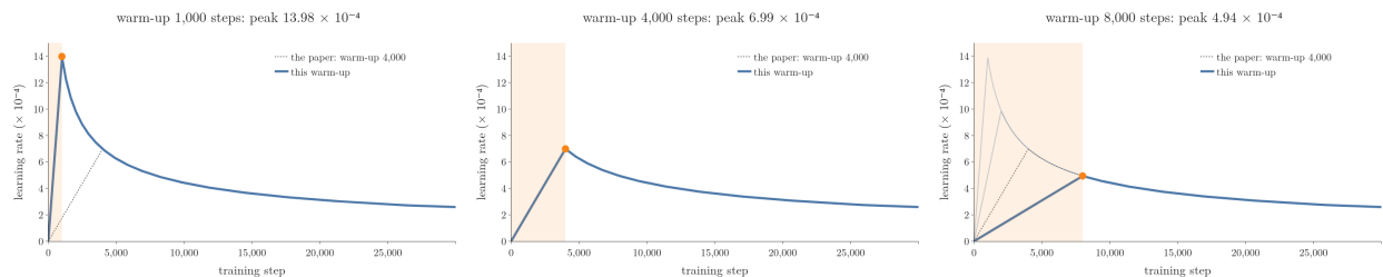
Figure 8: The same schedule as the warm-up length slides from 1,000 to 8,000 steps (first 30,000 steps shown). Orange band: the warm-up. Dotted: the paper’s 4,000. In the last frame the earlier curves stay as thin lines
