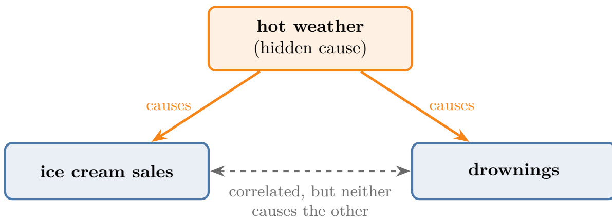
Figure 7: A hidden cause makes two features correlated
