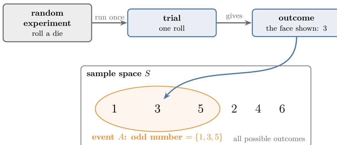
Figure 1: The five basic terms on one die roll
