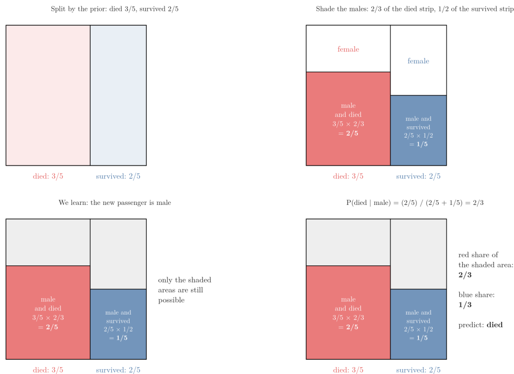
Figure 8: Bayes’ theorem as areas on the five passengers: the prior splits the square 3/5 and 2/5 , the likelihoods shade the male part of each strip, and the posterior 2/3 is the red share of the shaded area. Idea after 3Blue1Brown, “Bayes theorem, the geometry of changing beliefs”
