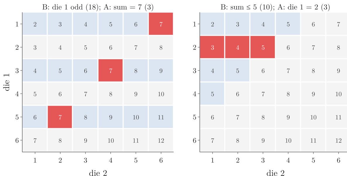
Figure 5: Two conditional probabilities on the 36 outcomes of two dice: blue = B , red = A inside B
