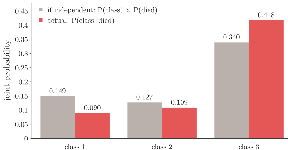
Figure 7: For each class, the actual P(\text{class, died}) (red) against the product P(\text{class}) \times P(\text{died}) that independence would give (grey)
