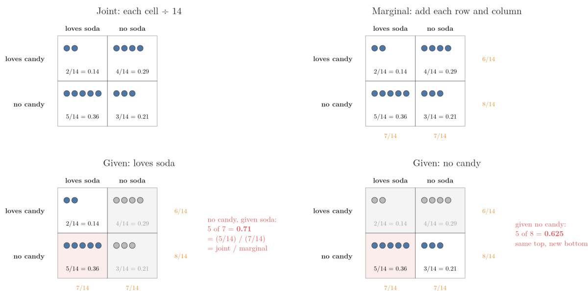
Figure 2: The same 14 people read four ways: each cell ÷ 14 is a joint probability; the row and column totals are marginal probabilities; knowing “loves soda” dims the other column and leaves 5 of 7; knowing “no candy” dims the other row and leaves 5 of 8. Idea after StatQuest, “Bayes’ Theorem, Clearly Explained!!!!”
