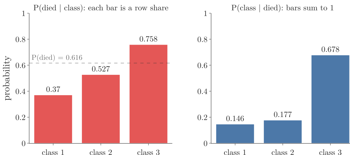
Figure 6: P(\text{died} \mid \text{class}) for each class (left) and P(\text{class} \mid \text{died}) (right)
