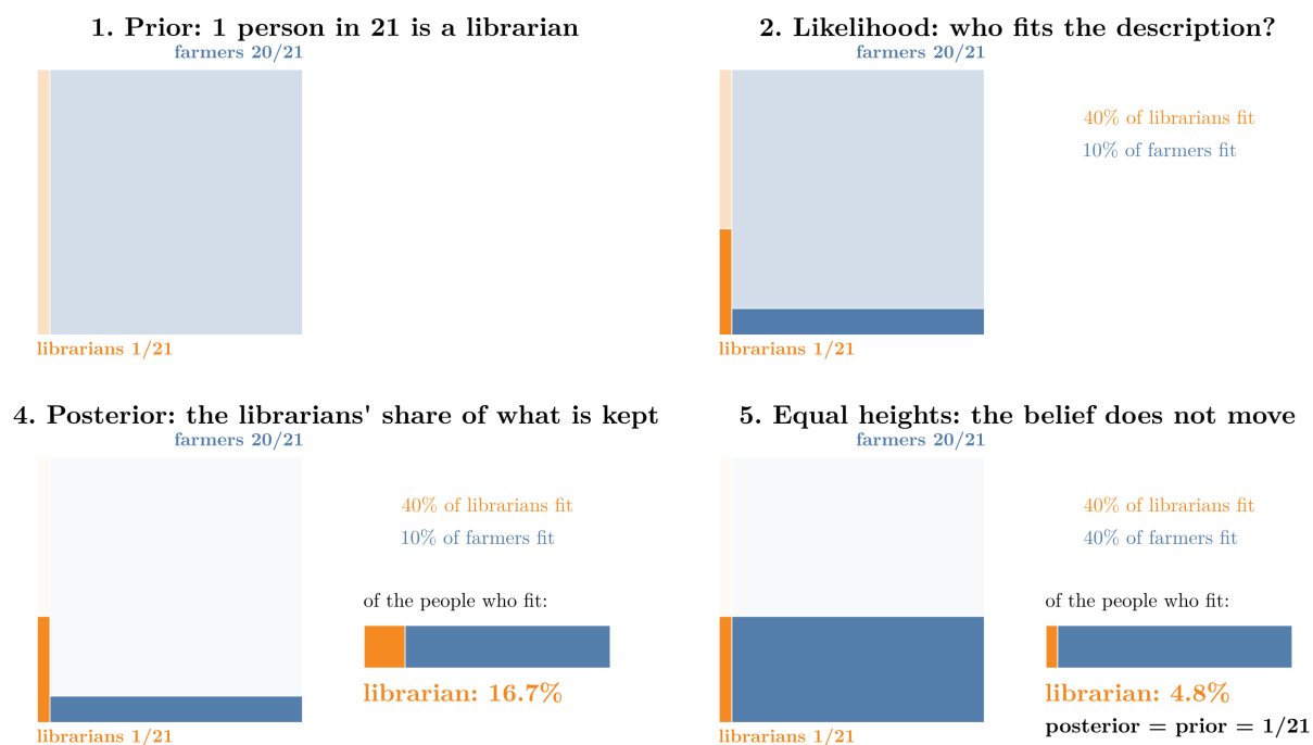
Figure 4: Bayes' theorem as areas, on the librarian numbers. The librarians are a strip of width 1/21 . The description keeps 40% of that strip and 10% of the farmers' strip. The bar on the right shows the librarians' share of what is kept: 16.7%. In the last step the farmers' height rises to 40%, and the share falls back to the prior, 4.8%. Idea after Sanderson (3Blue1Brown), "Bayes theorem, the geometry of changing beliefs".
