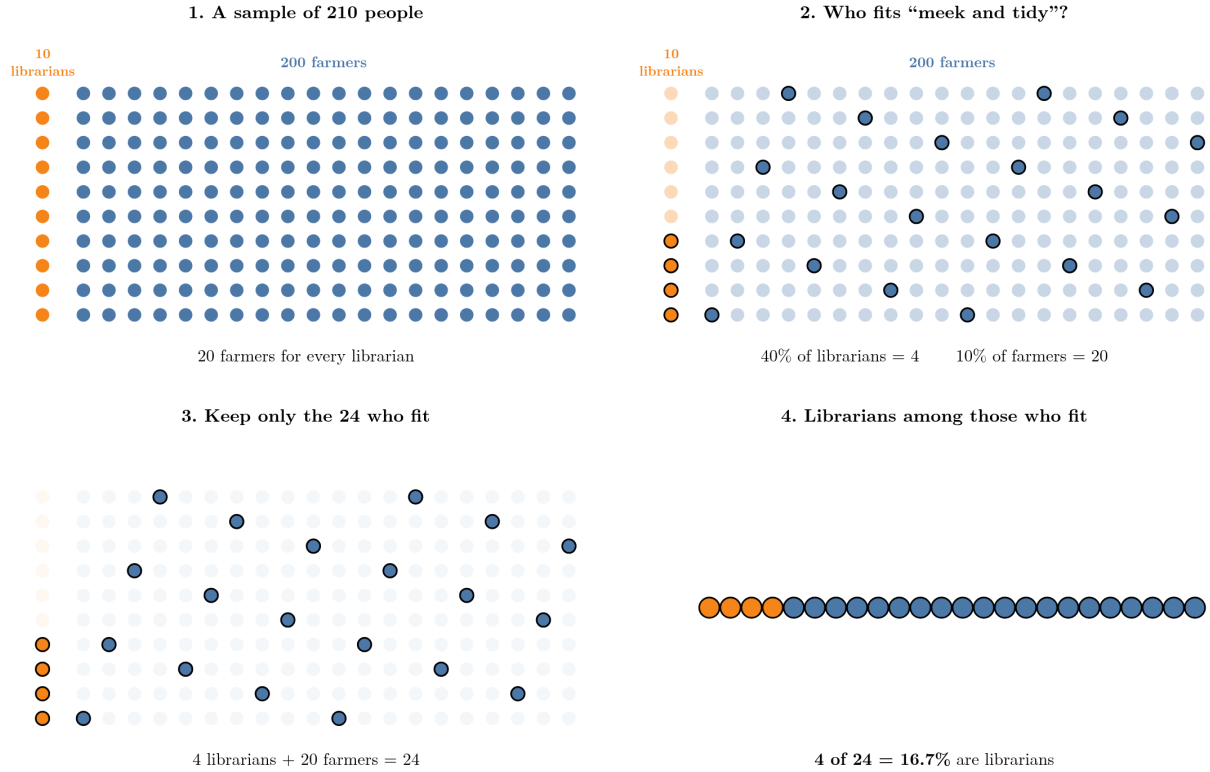
Figure 1: The puzzle as counts. 1: 10 librarians and 200 farmers. 2: the 4 librarians and 20 farmers who fit the description are outlined. 3: everyone else is ruled out. 4: of the 24 who fit, 4 are librarians, 16.7%. Idea after Sanderson (3Blue1Brown), “Bayes theorem, the geometry of changing beliefs”.
