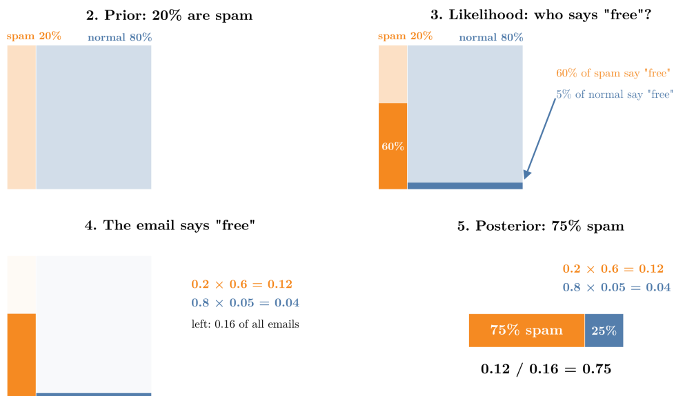
Figure 5: Bayes’ theorem as areas, on the spam numbers. Prior: a 20% spam strip. Likelihood: the “free” share inside each strip. Evidence: only the two dark pieces remain (0.12 and 0.04). Posterior: rescaled to fill the whole, spam is 0.12 / 0.16 = 75\% . Idea after Sanderson (3Blue1Brown), “Bayes theorem, the geometry of changing beliefs”.
