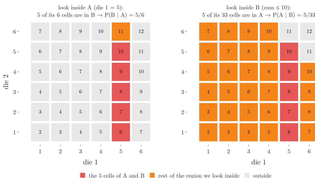
Figure 3: The proof on the 36 outcomes of two dice. Left: inside A , 5 of 6 cells are in B , so P(A \text{ and } B) = 5/6 \times 6/36 . Right: inside B , 5 of 33 cells are in A , so P(A \text{ and } B) = 5/33 \times 33/36 . Both equal 5/36
