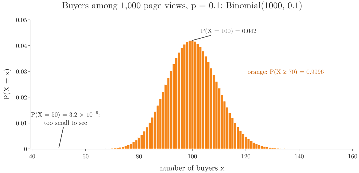
Figure 6: The PMF of the number of buyers among 1,000 page views with p = 0.1 . The peak is P(X = 100) = 0.042 ; P(X = 50) is invisible; the orange bars, 70 and above, hold 0.9996 of the probability.
