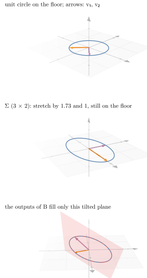
Figure 8: The SVD of the 3 \times 2 matrix B in 3D. The unit circle lies on the floor (third coordinate 0) with \mathbf{v}_1 (orange) and \mathbf{v}_2 (purple). V^T turns it on the floor, \Sigma stretches it into an ellipse of axes 1.73 and 1, still on the floor, and U tilts it up onto the plane of B 's outputs (red). The dashed curve is B applied in one step. 2D-to-3D picture after 3Blue1Brown, “Nonsquare matrices as transformations between dimensions”
