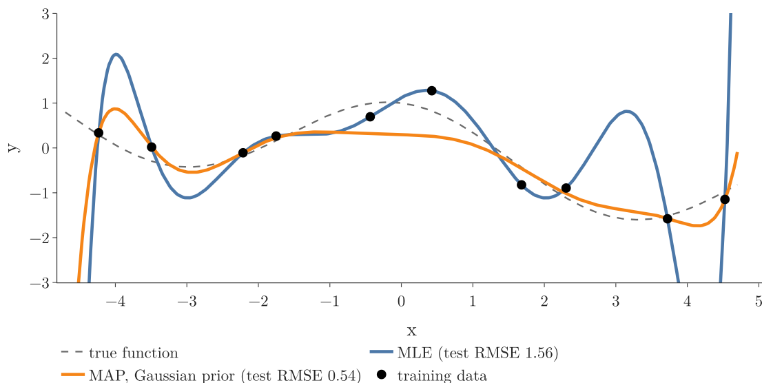
Figure 9: Degree-9 polynomial on ten points: maximum likelihood versus MAP with a Gaussian prior
