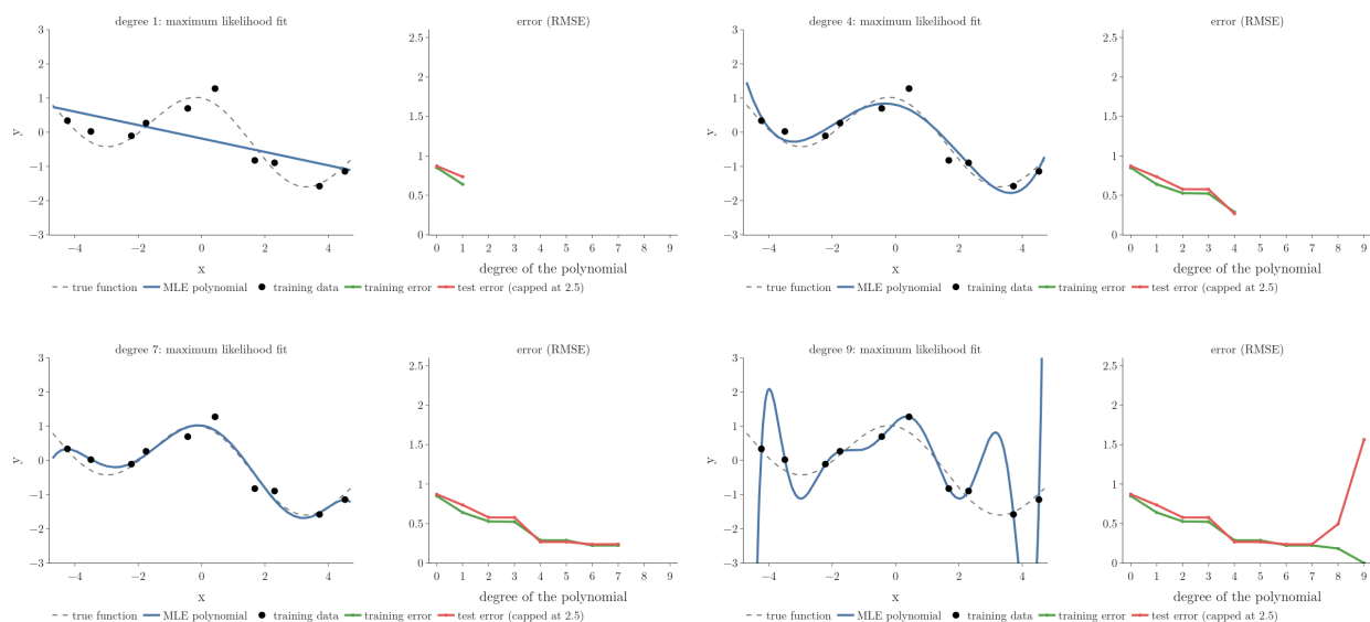
Figure 8: Maximum likelihood polynomials of degree 0 to 9 on ten points. Right: the training error falls to 0 while the test error, after a minimum, shoots up
