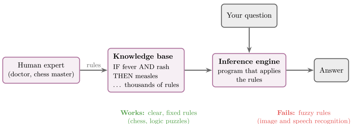
Figure 5: How an expert system works
