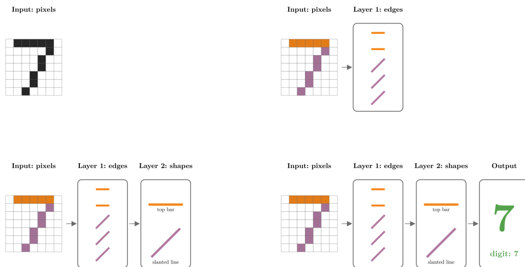
Figure 9: Layers of a neural network recognising a handwritten 7
