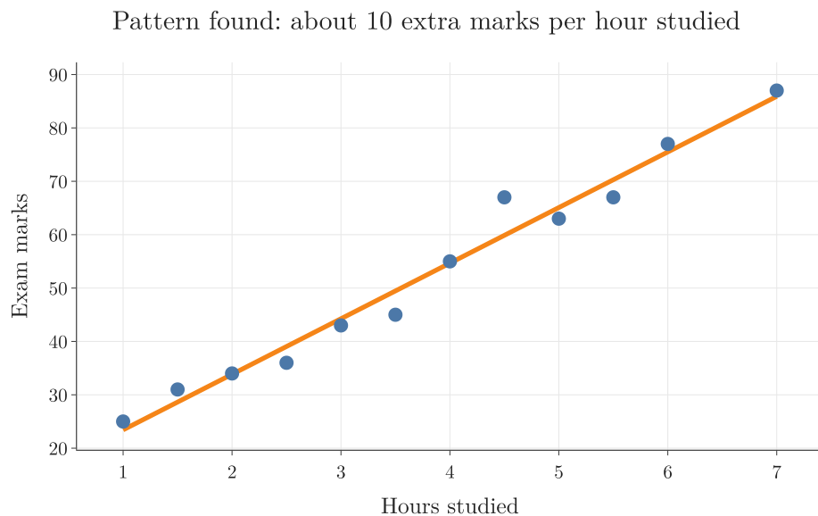
Figure 6: A pattern in data: marks rise with hours studied (example data)
