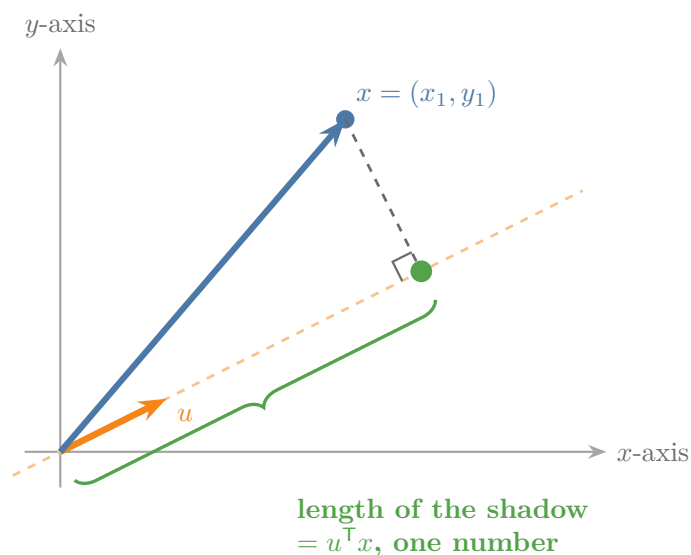
Figure 1: Projecting a point onto a unit vector
