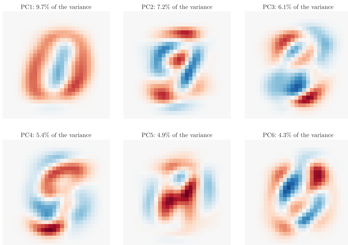
Figure 7: The first six eigenvectors of MNIST, each reshaped to 28 \times 28 (PCA fitted on all 70,000 images). Red pixels count positively, blue negatively.
