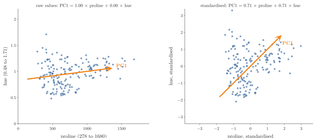
Figure 4: PCA on two wine features. Left: raw values; PC1 is almost pure proline, only because proline’s numbers are about a thousand times bigger. Right: after standardising, PC1 uses both features in equal parts. Idea after StatQuest, “PCA - Practical Tips”.
