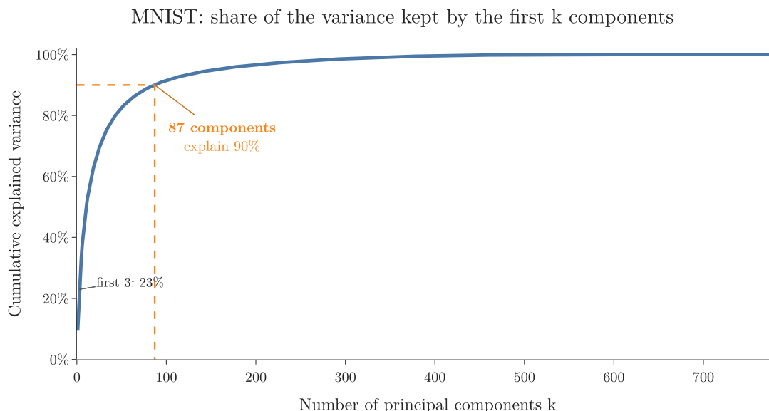
Figure 8: Cumulative explained variance of MNIST's components
