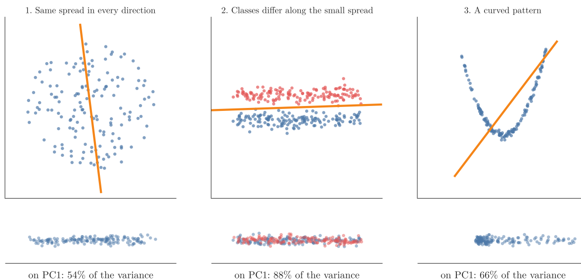
Figure 9: Three cases where PCA does not help
