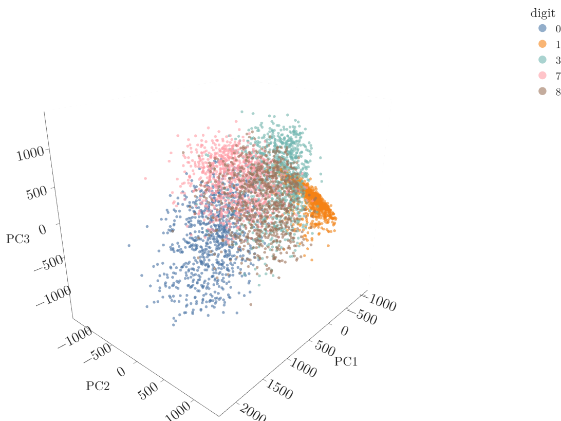
Figure 6: Digits 0, 1, 3, 7 and 8 on PC1, PC2 and PC3
