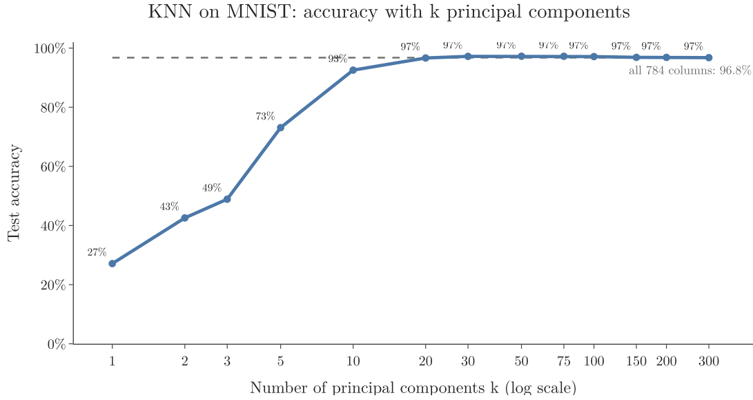
Figure 3: KNN accuracy on MNIST with k principal components; the dashed line is KNN on all 784 pixels
