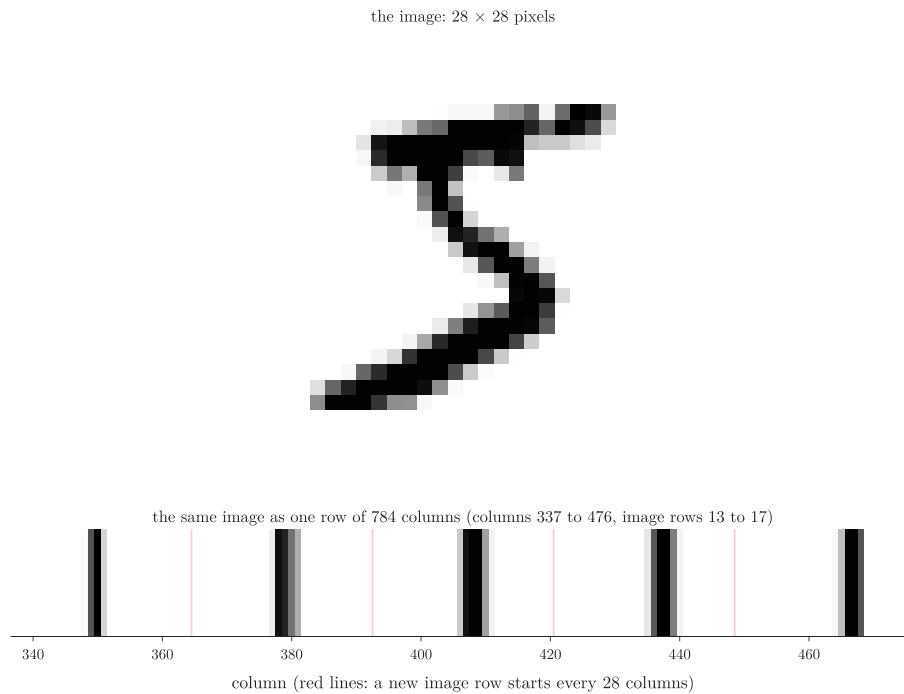
Figure 1: The first MNIST training image, a 5, as a 28 \times 28 picture (top) and as part of its row of 784 columns (bottom). Every 28 columns, a new image row starts (red lines).
