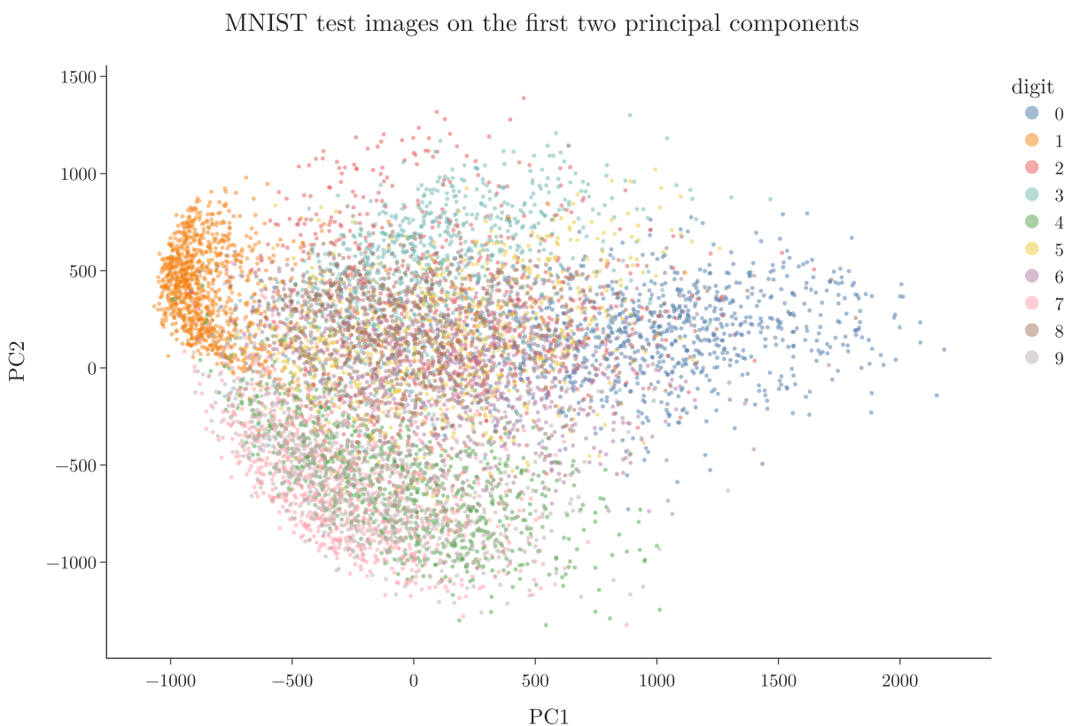
Figure 5: MNIST test images on PC1 and PC2
