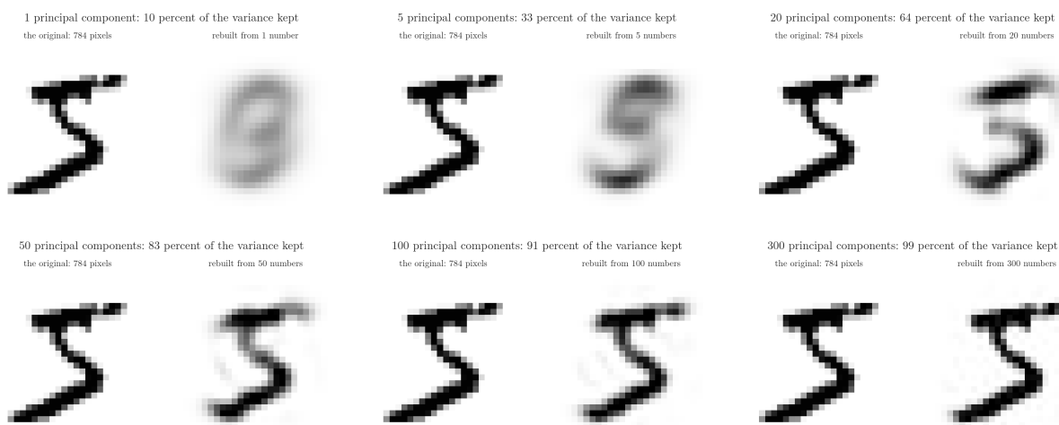
Figure 2: One MNIST image rebuilt from its first 1, 5, 20, 50, 100 and 300 principal components (PCA fitted on all 70,000 images). Left of each pair: the original 784 pixels.
