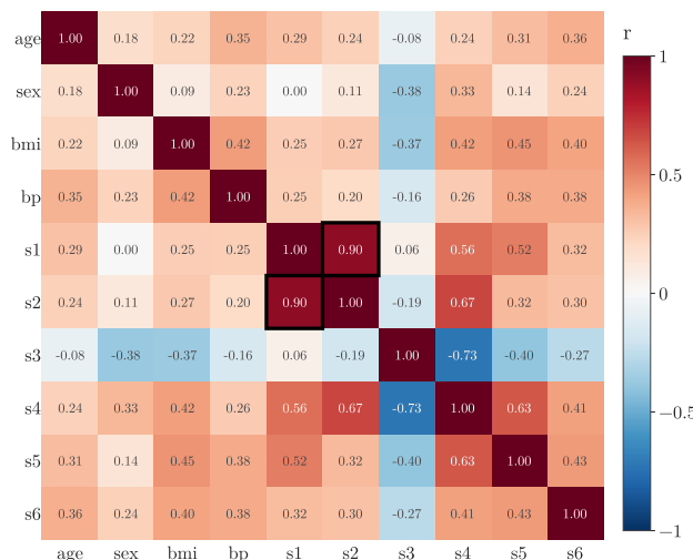
Figure 1: Correlation between the 10 diabetes features on the 353 training patients; s1 and s2 (outlined) are at 0.90
