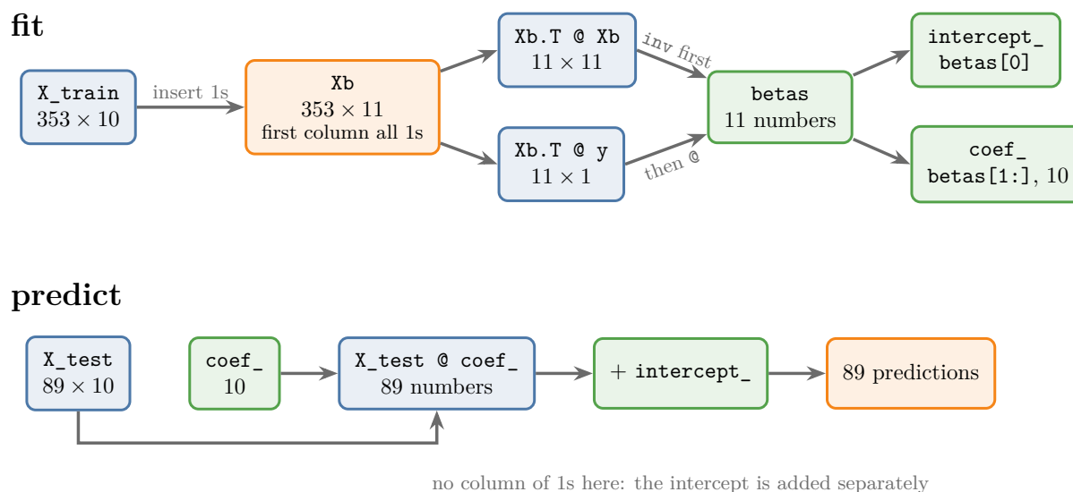
Figure 3: The shapes through MyMLR: fit turns the 353 \times 10 training data into 11 numbers, the intercept and 10 coefficients; predict turns the 89 \times 10 test data into 89 predictions
