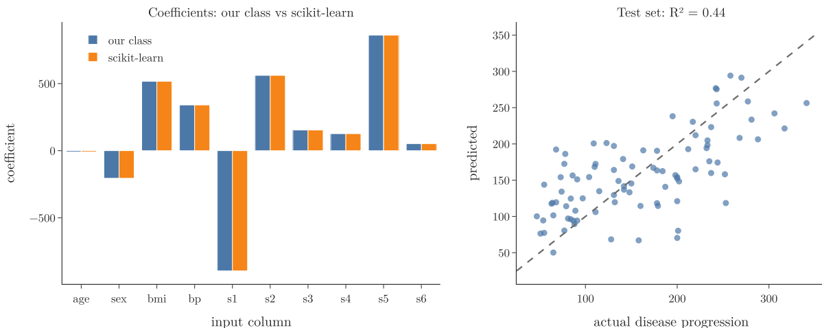
Figure 4: Coefficients of our class and scikit-learn; predicted against actual on the test set
