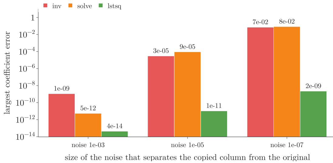
Figure 5: Largest coefficient error of inv, solve and lstsq as the copied column gets closer to the original (log scale); lstsq stays accurate
