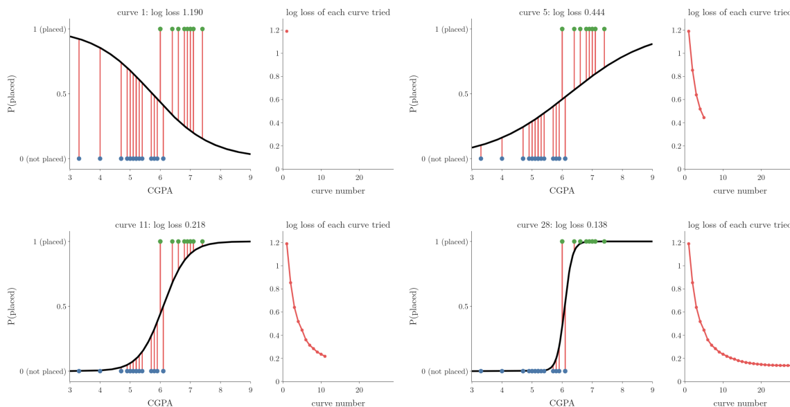
Figure 7: Thirty students (green: placed, blue: not placed) and a candidate sigmoid curve. Each red bar is the gap between a student and the curve: 1 minus the probability the curve gives to the student’s true class. From curve to curve the bars shrink and the log loss falls from 1.190 to 0.138, where it stops falling. Idea after StatQuest, “Logistic Regression Details Pt 2: Maximum Likelihood”; the data and curves are our own
