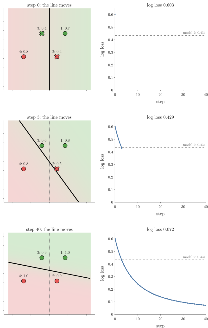
Figure 8: Gradient descent on the log loss of the four points, starting from model 1 (dotted line). Left: the decision boundary ( P(\text{green}) = 0.5 ) turns; the labels give each point's probability for its true colour. Right: the log loss per step, with model 2's 0.434 dashed. Key frames: steps 0, 3 and 40.
