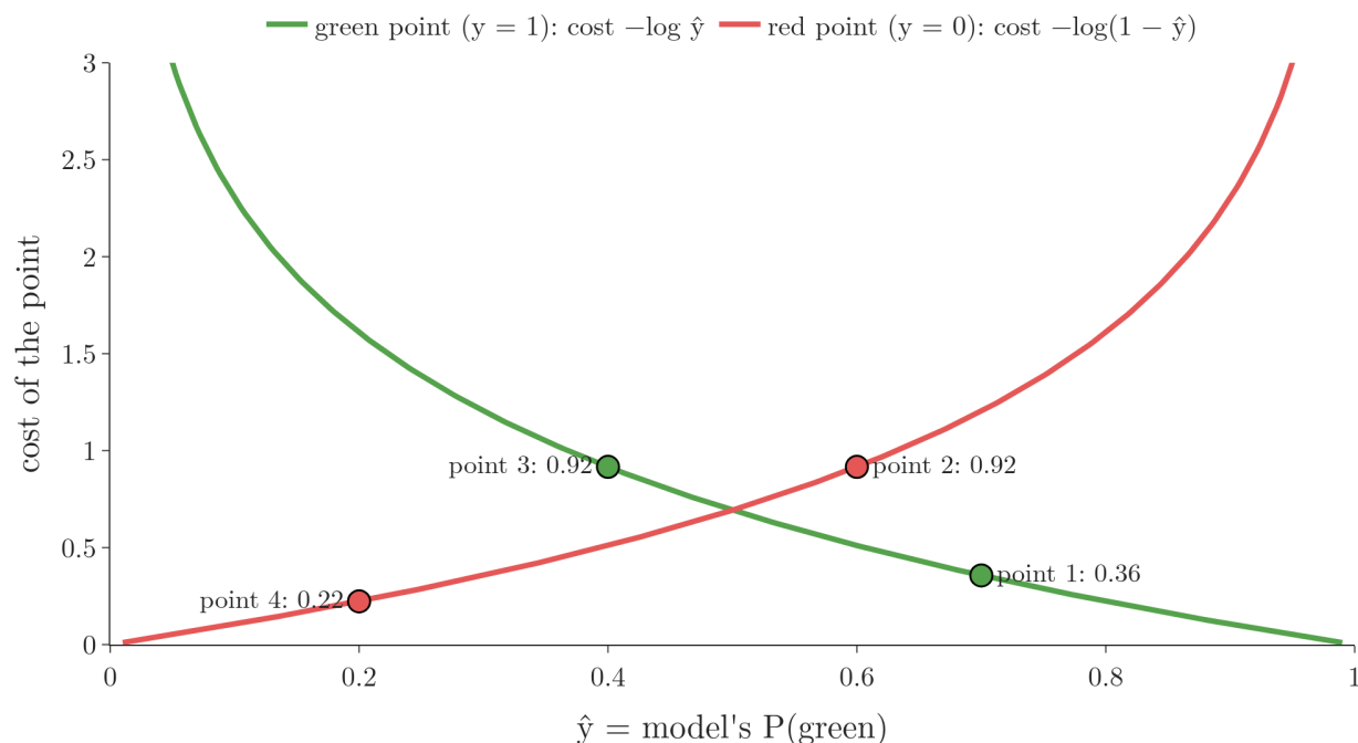
Figure 6: The one formula draws two cost curves: green points pay -\log \hat{y} , red points pay -\log(1 - \hat{y}) . Model 1's four points sit on their own curves; their costs add up to 2.41.
