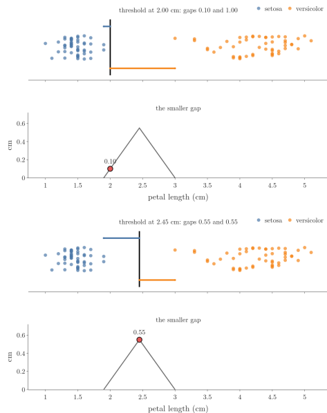
Figure 2: A threshold slides across the gap between the longest setosa petal (1.9 cm) and the shortest versicolor petal (3.0 cm). Top: its distance to the nearest flower of each species. Bottom: the smaller of the two distances, which peaks at the midpoint, 2.45 cm. Idea after StatQuest, “Support Vector Machines Part 1 (of 3): Main Ideas!!!”, shown there on mouse weights.
