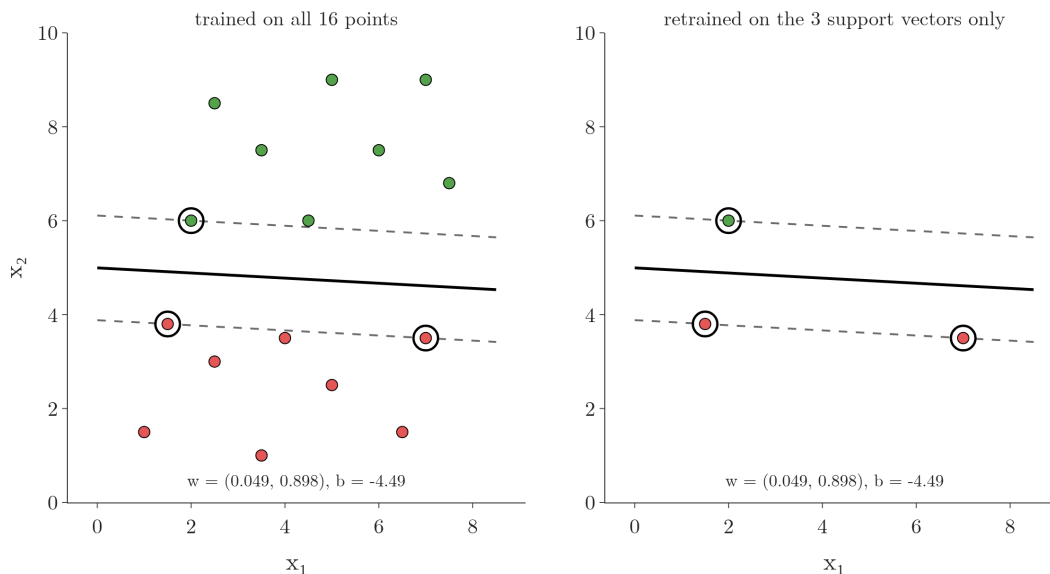
Figure 6: The hard-margin SVM trained on all 16 points (left) and retrained on its 3 ringed support vectors only (right): the same line and margin, w = (0.049, 0.898) , b = -4.49 .
