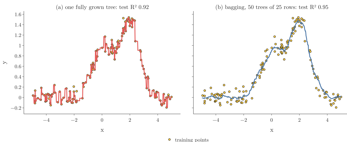
Figure 2: (a) One fully grown regression tree; (b) a bagging regressor of 50 trees, each trained on 25 observations drawn with replacement
