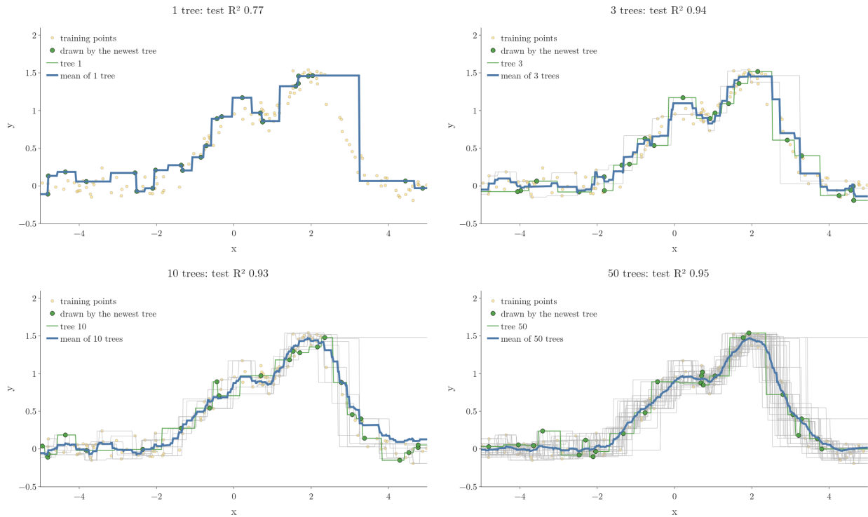
Figure 3: The bagging regressor built one tree at a time: every tree so far (grey), the newest tree and its 25 drawn points (green), and the mean of the trees, the bagging prediction (blue)
