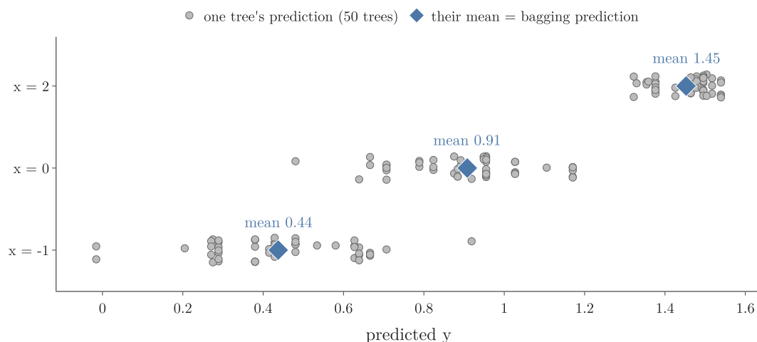
Figure 1: Aggregation in a bagging regressor: at three inputs x , each of the 50 bagged trees of section 3 returns a number (grey dots); the bagging prediction is their mean (blue diamond)
