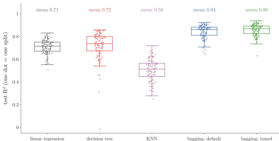
Figure 4: Test R^2 of five regressors on the same 100 random splits of the Boston data: each dot is one split, the box holds the middle half, and the number on top is the mean
