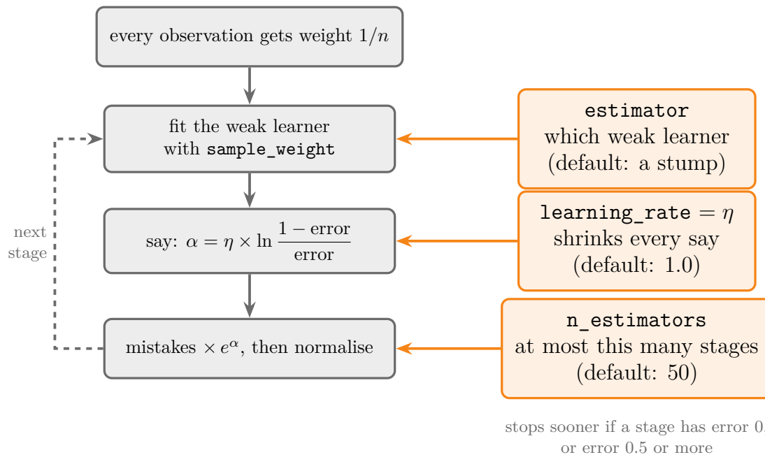
Figure 2: The scikit-learn AdaBoost loop (SAMME) and the three hyperparameters: estimator sets the weak learner, learning_rate scales every alpha, n_estimators caps the number of stages
