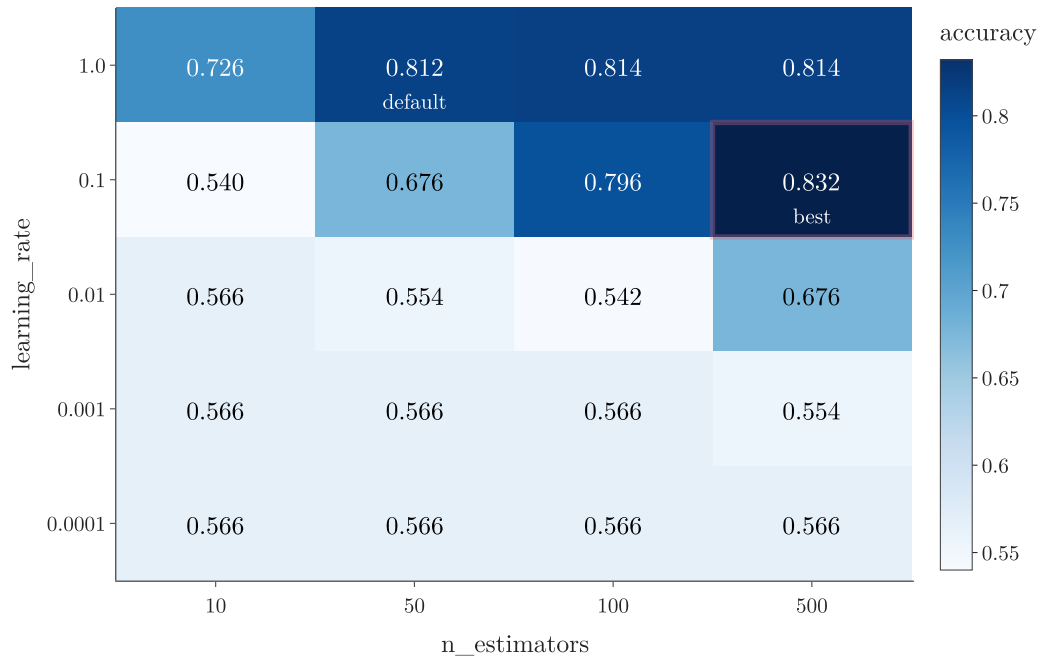
Figure 6: 10-fold cross-validated accuracy of every pair in the grid; the red box is the best pair, 500 stumps at learning rate 0.1
