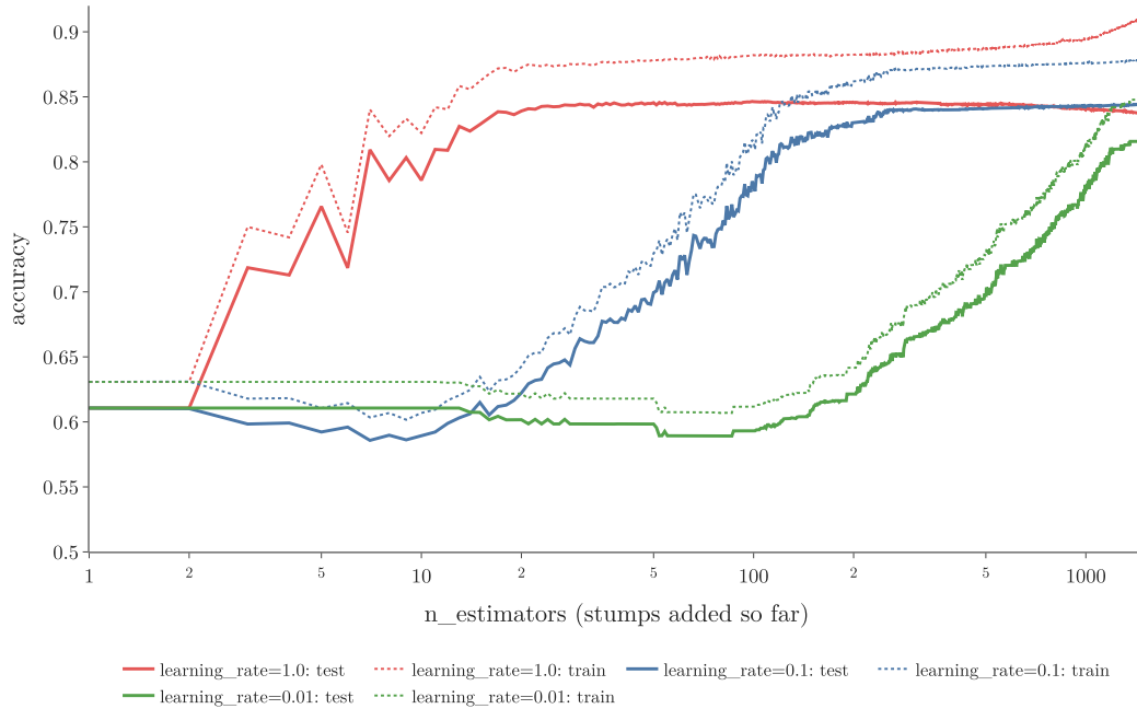
Figure 5: Training (dotted) and test (solid) accuracy as stumps are added, for three learning rates, averaged over 20 datasets; the horizontal axis is logarithmic
