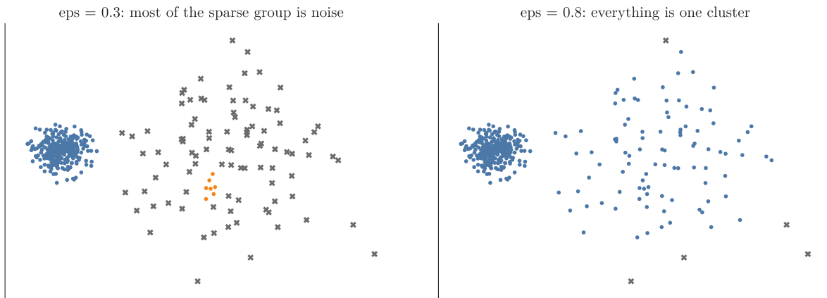
Figure 9: DBSCAN on a dense group and a sparse group: no single eps works
