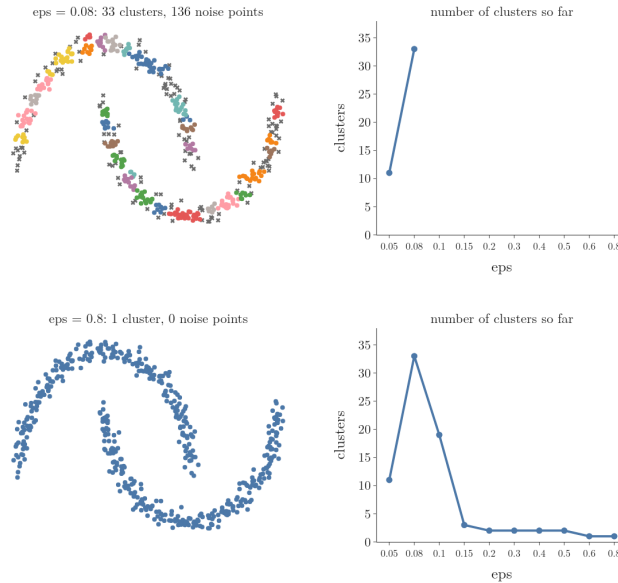
Figure 8: DBSCAN on the two moons as eps grows from 0.05 to 0.8, MinPts = 5. Left: the clusters found (grey crosses: noise). Right: the number of clusters for every eps tried so far.
