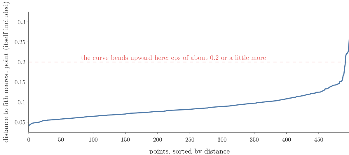
Figure 10: k-distance plot for the moons with MinPts = 5: the curve bends upward at about 0.2
