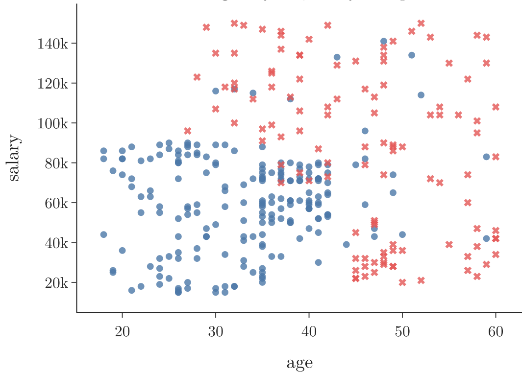
Raw: age in years, salary in rupees
