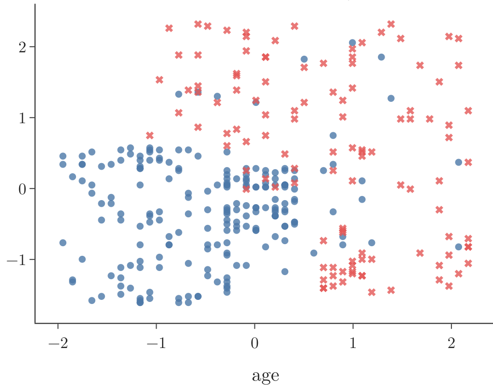
Standardized: both mean 0, std 1
