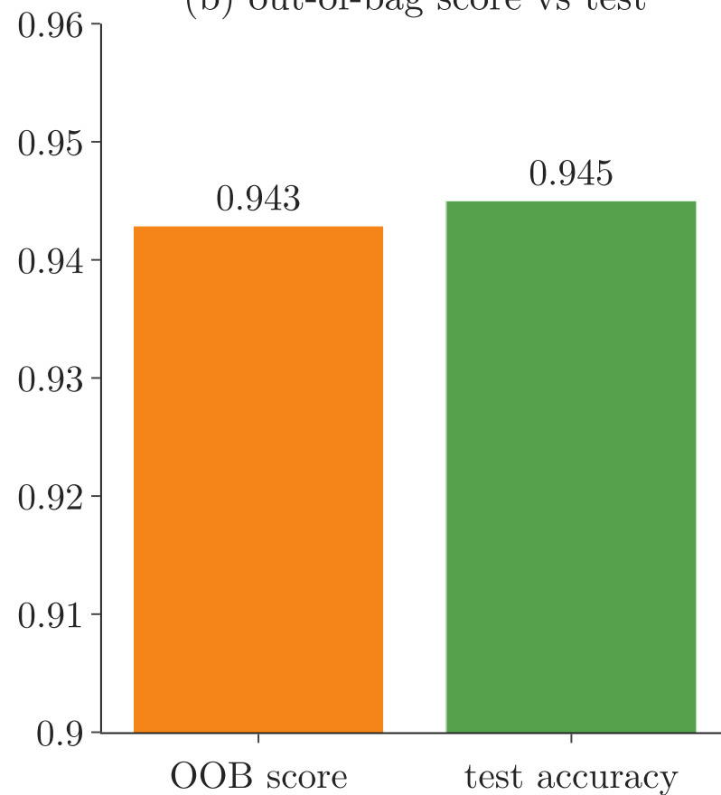
(b) out-of-bag score vs test
