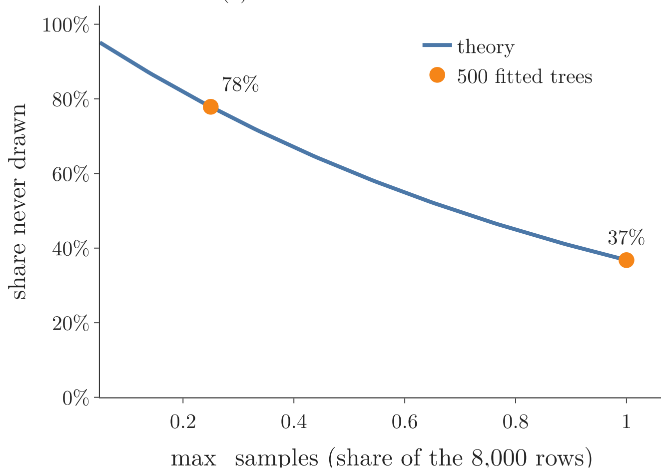
(a) share of rows a tree never sees
