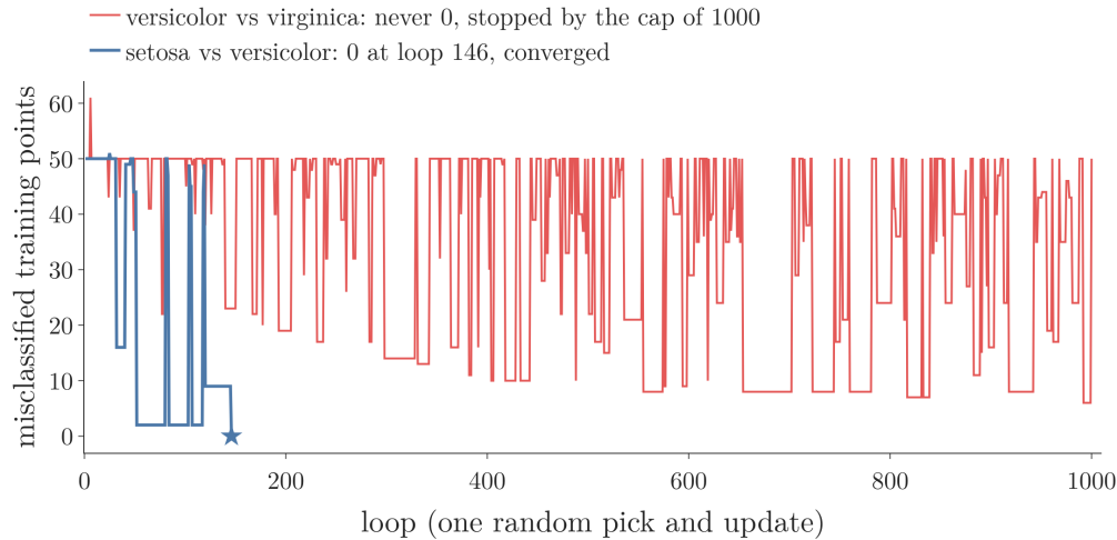
Figure 2: The perceptron trick on two pairs of Iris species (petal length and width, 100 flowers each, learning rate 0.1), counting the misclassified training points after every loop
