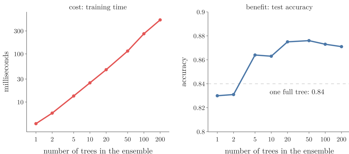
Figure 7: Bagging ensembles of 1 to 200 full-depth trees on the two-moons data. Left: training time (log scale). Right: test accuracy, averaged over 5 seeds; dashed: one full tree
