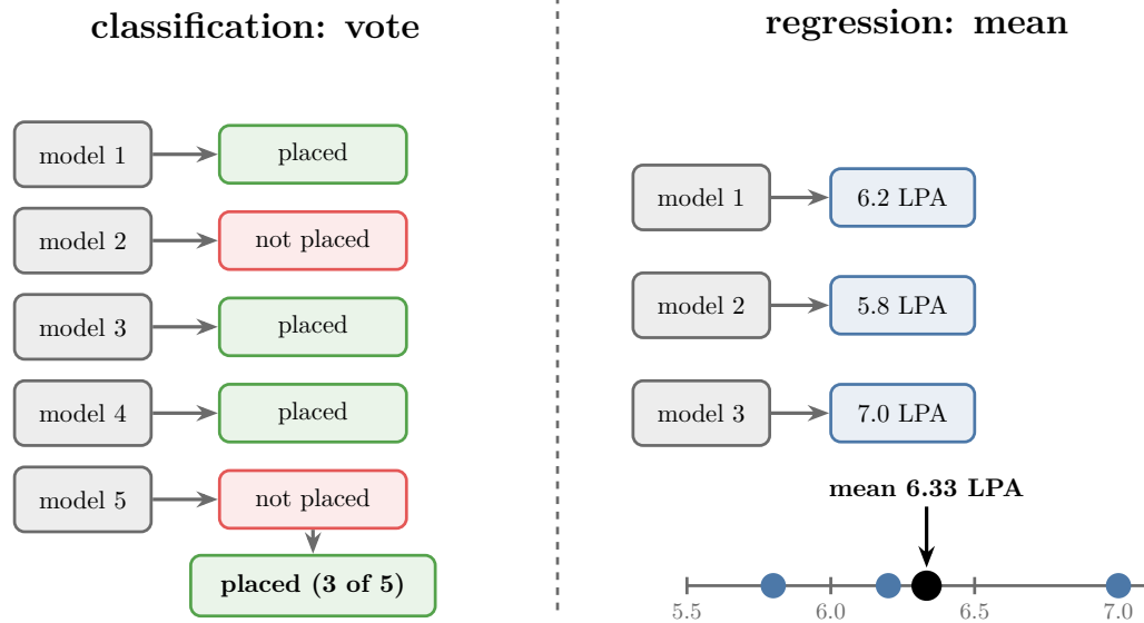
Figure 3: Left: five models vote, 3 for placed and 2 for not placed, so the ensemble says placed. Right: three models predict 6.2, 5.8 and 7.0 LPA, and the ensemble returns their mean, 6.33 LPA
