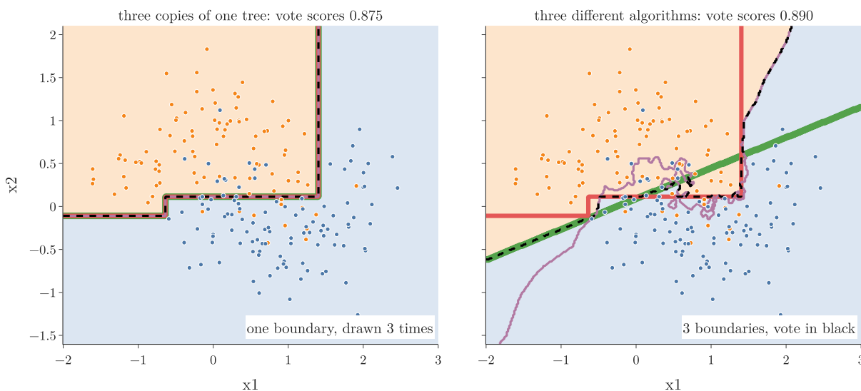
Figure 2: Left: three copies of one depth-3 tree, trained on the same data, and their vote. Right: logistic regression (green), a depth-3 tree (red) and KNN with k = 5 (purple), and their vote (black dashed). Test accuracy of the vote in each title
