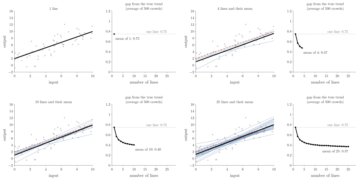
Figure 6: Lines added one at a time, each fitted to 10 random points of the same data. Left: the lines (blue), their mean (black) and the true trend (red dashed). Right: the gap between the mean line and the true trend, averaged over 500 crowds
