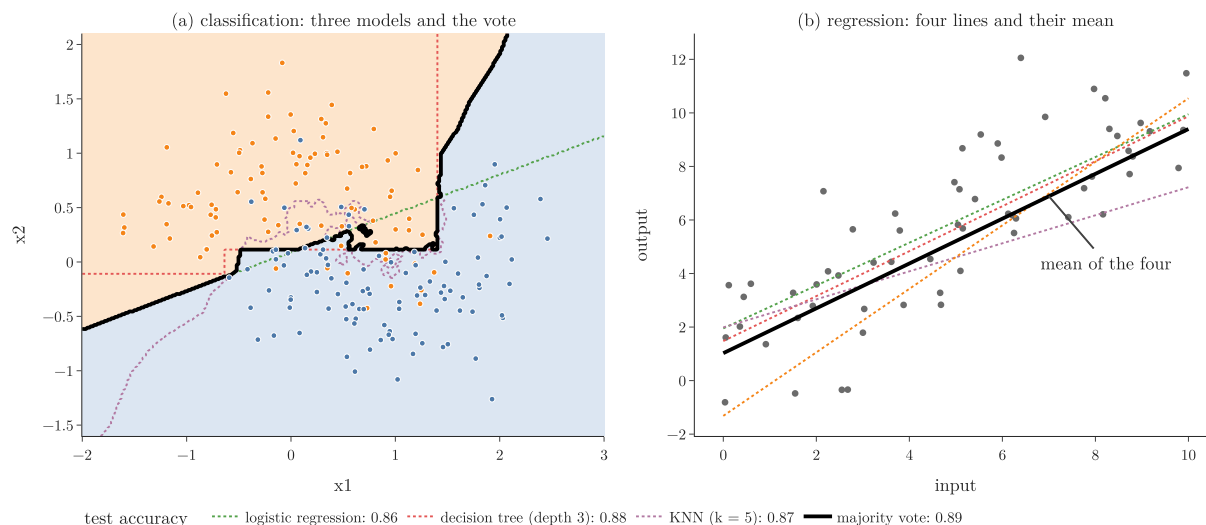
Figure 5: (a) Three classifiers' decision boundaries (dotted) and their majority-vote decision boundary (black) on two-moons data; (b) four lines, each fitted to 10 random points, and their mean
