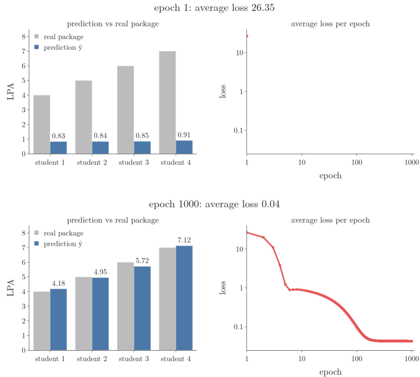
Figure 6: The full algorithm for 1,000 epochs: predictions against real packages (left) and the average loss of each epoch (right)
