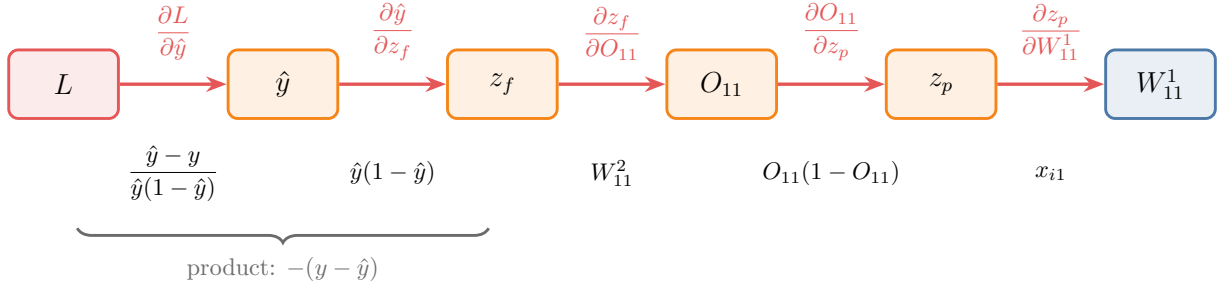
Figure 6: The chain from the loss to a first-layer weight in the classification network: each arrow multiplies by its local derivative
