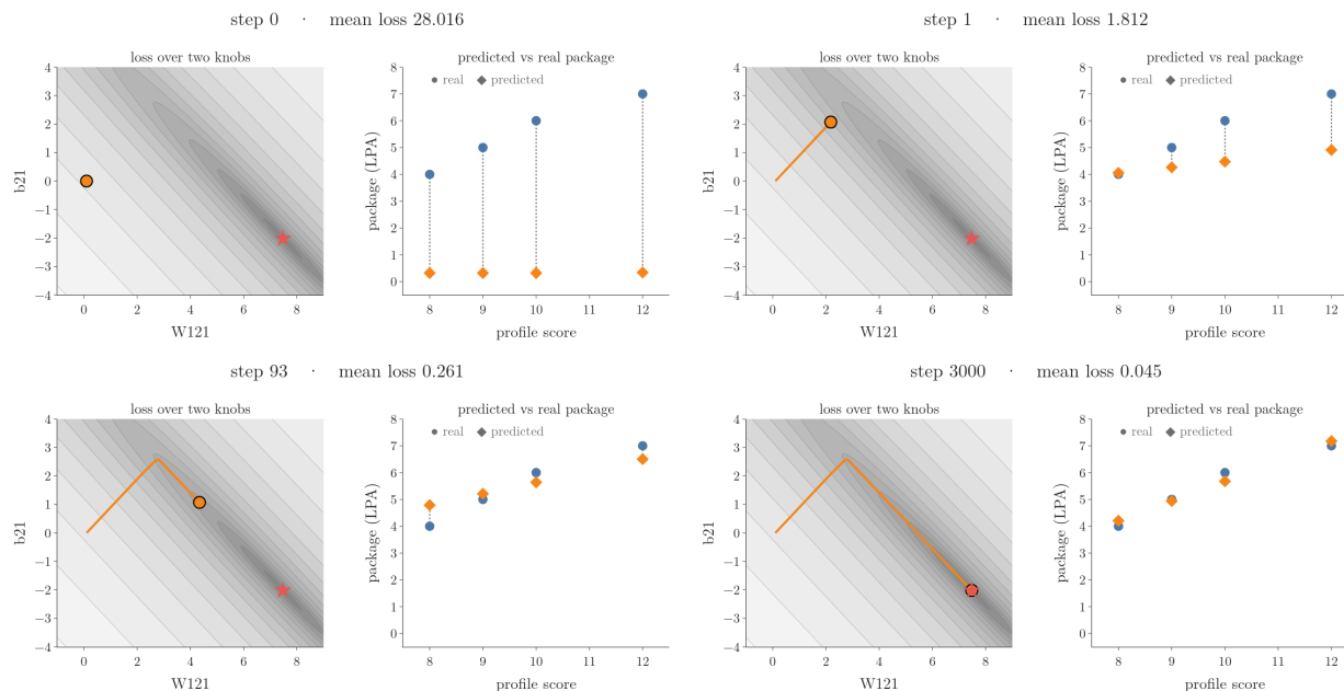
Figure 6: Gradient descent on two of the nine knobs at once, W_{21}^1 and b_{21} , over all four students; the other seven stay at their starting values. Left: the path on the contours of the mean loss (the star is the lowest point). Right: the predicted packages (diamonds) move onto the real ones (dots). Learning rate 0.2.
