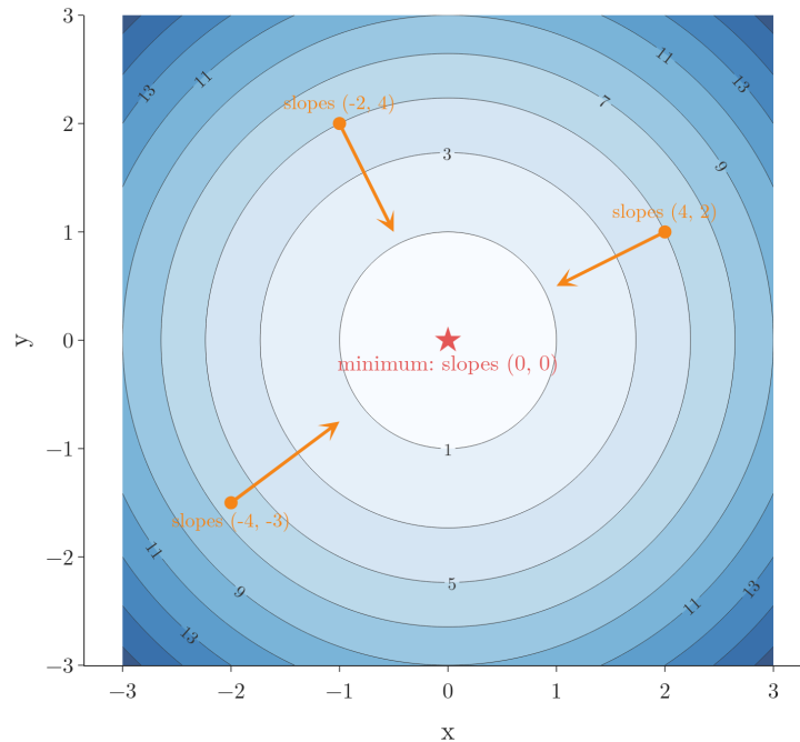
Figure 4: Contours of z = x^2 + y^2 . At three points the arrow is minus the two slopes; only at the star are both slopes zero
