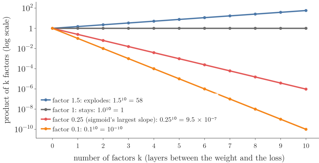
Figure 2: The product of k equal factors as k grows, log scale
