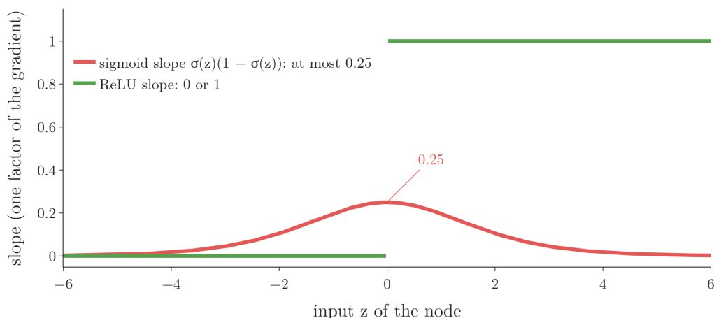
Figure 5: The slope of each activation against its input: sigmoid (red) never exceeds 0.25; ReLU (green) is exactly 0 or 1
