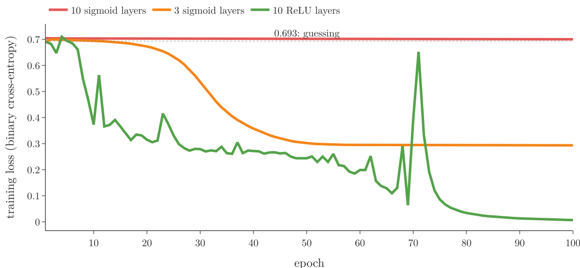
Figure 3: Training loss over 100 epochs: 10 sigmoid layers stay at the guessing level; 3 sigmoid layers and 10 ReLU layers learn
