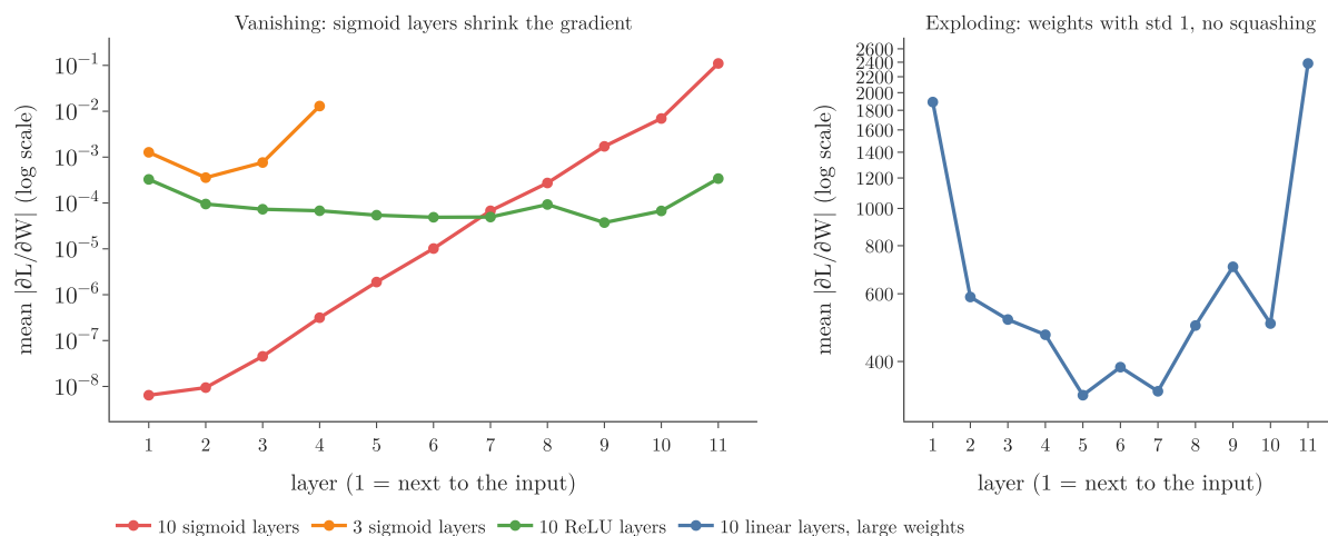
Figure 1: Mean size of the gradient of each layer’s weights at the start of training. Left: 10 sigmoid layers (red) shrink it about 17-million-fold towards the input. Right: large weights without squashing make every gradient huge
