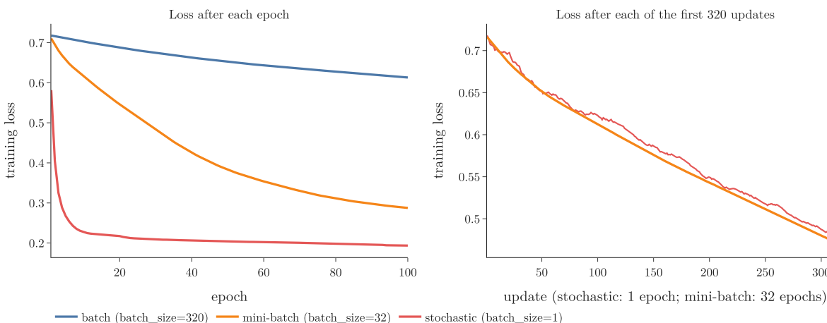
Figure 6: Left: training loss per epoch over 100 epochs. Right: loss on all 320 training observations after each single update
