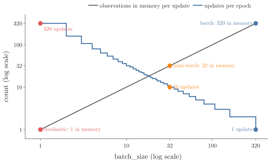
Figure 7: The two costs of batch_size on our 320 training observations (both axes log scale). Grey: observations that must sit in memory for one update. Blue: updates per epoch, \lceil 320/\text{batch size} \rceil .
