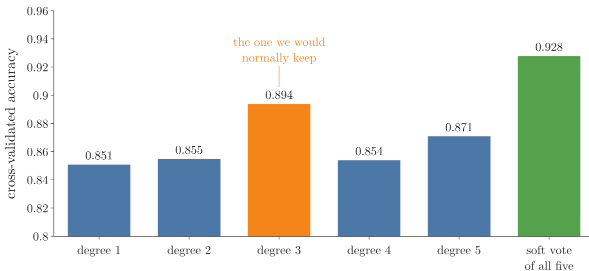
Figure 6: Polynomial-kernel SVMs of degree 1 to 5, each alone, and all five in one soft vote (10-fold cross-validation)
