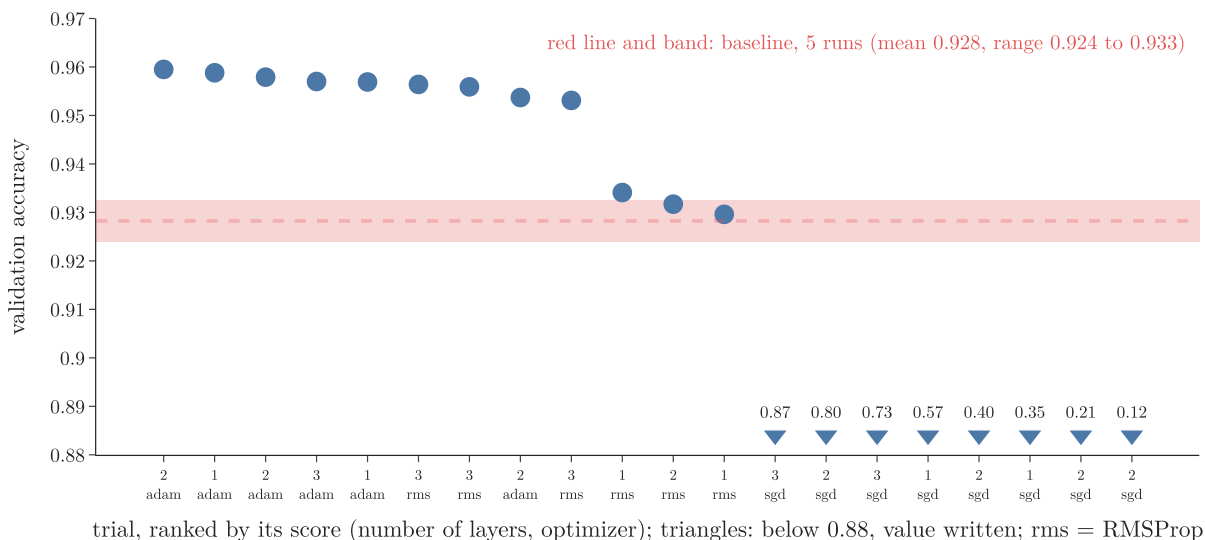
Figure 8: MNIST: validation accuracy of the 20 trials, ranked, labelled with layers and optimizer; trials below 0.88 are drawn as triangles with their value. Red band and dashed line: the hand-made guess, 5 seeds
