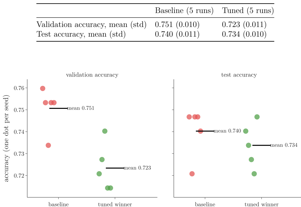
Figure 7: Pima diabetes: the baseline and the tuned winner, each retrained with 5 seeds. One dot per run; the black bar is the mean.
