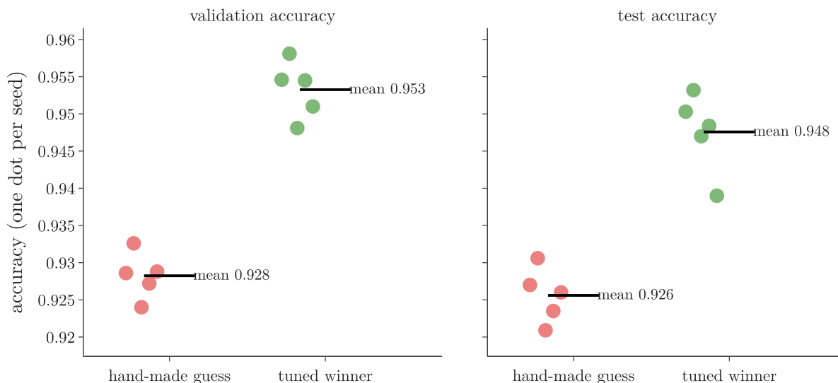
Figure 9: MNIST: the hand-made guess and the tuned winner, each retrained with 5 seeds. One dot per run; the black bar is the mean.
