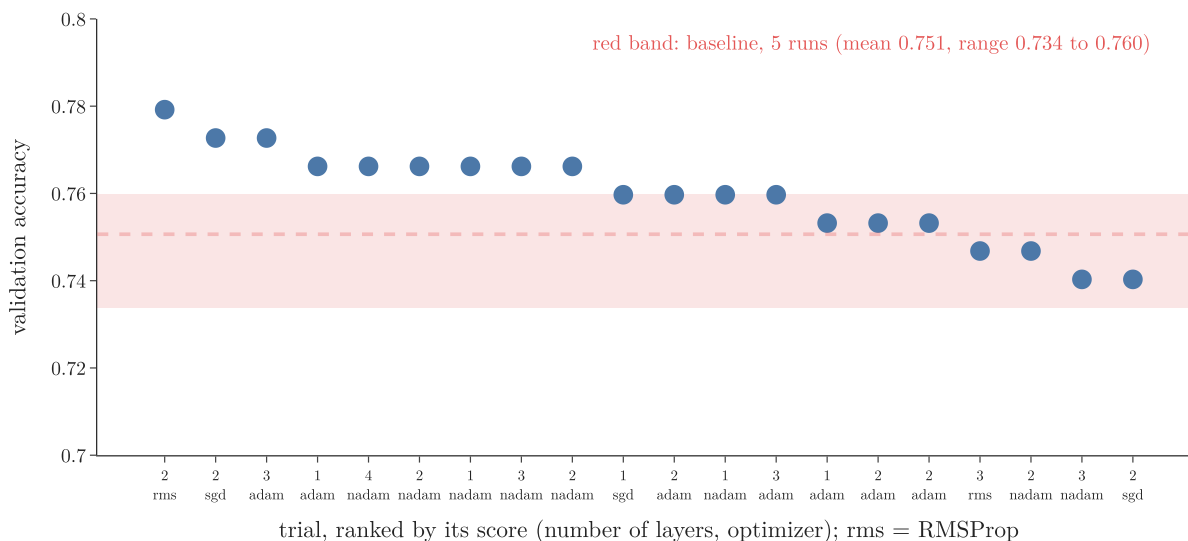
Figure 6: Validation accuracy of the 20 trials (best epoch of 100), ranked, each labelled with its number of layers and optimizer. Red band and dashed line: the baseline after 100 epochs, 5 seeds
