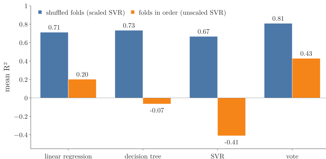
Figure 5: Mean R^2 with shuffled folds (blue) and with folds in order (orange), per model
