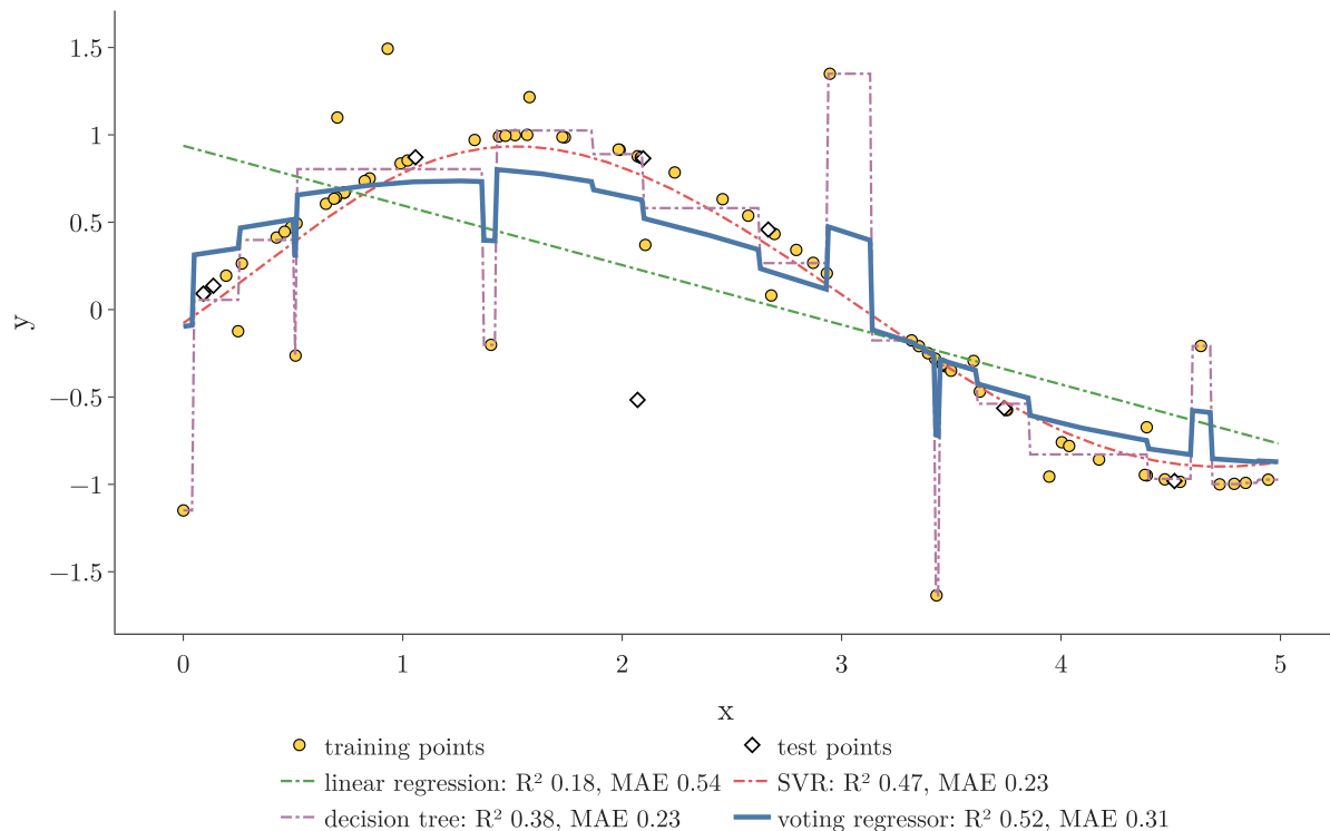
Figure 2: Three base regressors (dash-dot) and the voting regressor (solid blue) on noisy sine data; legend gives R^2 and MAE on the 8 test points
