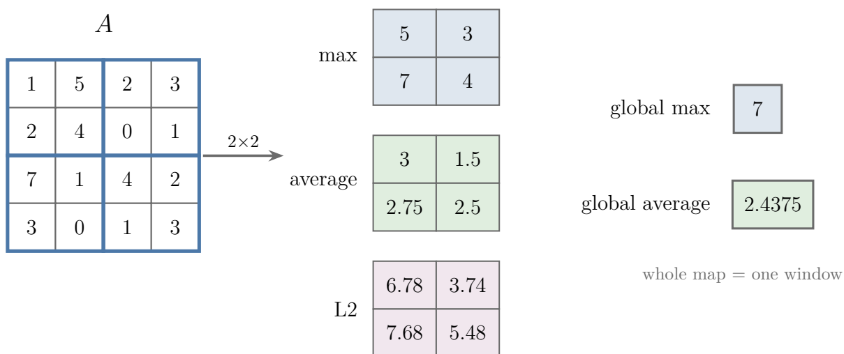
Figure 7: The map of section 4.3 summarised by max, average and L2 pooling ( 2 \times 2 , stride 2), and by global max and global average pooling.
