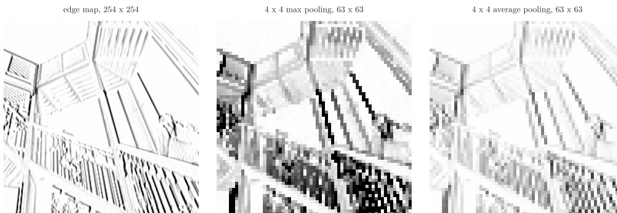
Figure 6: The vertical-edge map of a photo (left), after 4 \times 4 max pooling (middle) and after 4 \times 4 average pooling (right), on the same colour scale. Max pooling keeps the edges strong; averaging fades them
