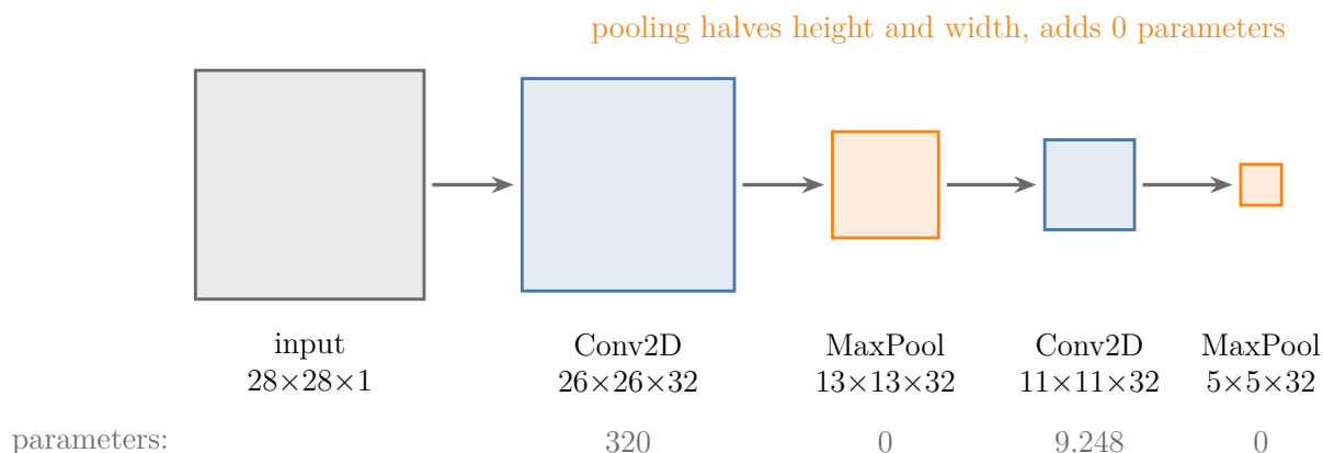
Figure 4: The output of each layer of the model above, drawn to scale (side = height of the map), with its parameter count.
