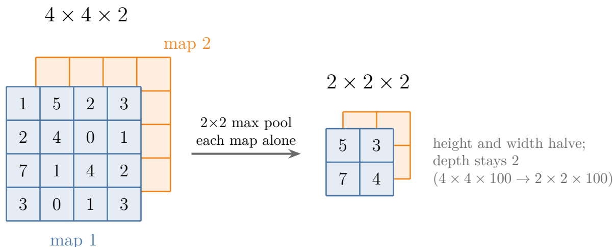
Figure 3: Pooling a 4 \times 4 \times 2 volume: each feature map is pooled on its own. The front map is the example of section 4.3.
