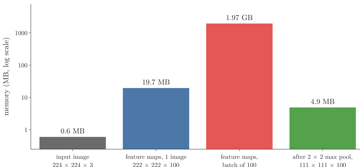
Figure 2: Memory of one input image, of the feature maps one convolution layer of 100 filters makes from it, of those maps for a batch of 100 images, and of one image’s maps after 2 \times 2 max pooling (section 7.1). Log scale; 4 bytes per number.
