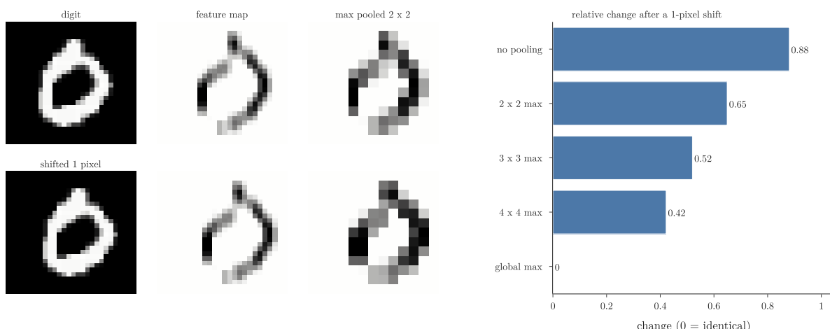
Figure 5: Left: a digit and the same digit shifted 1 pixel right, their feature maps (vertical-edge filter and ReLU) and 2 \times 2 max-pooled maps. Right: the relative change caused by the shift, averaged over 1,000 test digits; 0 means identical
