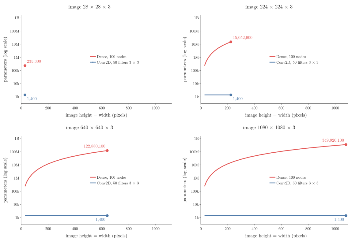
Figure 3: The image grows from 28 \times 28 \times 3 to 1080 \times 1080 \times 3 . Blue: parameters of a Conv2D layer of 50 filters of 3 \times 3 . Red: parameters of a Dense layer of 100 nodes on the flattened image. Log scale.
