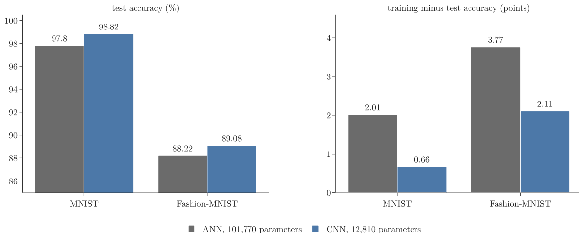
Figure 4: Mean of 3 seeds. Left: test accuracy (the axis starts at 85%). Right: training accuracy minus test accuracy, a measure of overfitting. The CNN, with 8 times fewer parameters, is more accurate and overfits less on both datasets
