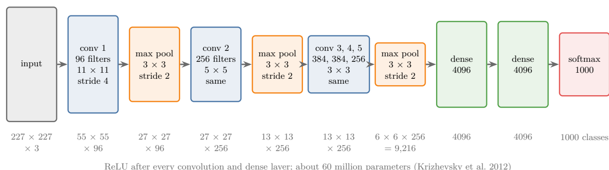
Figure 4: AlexNet: five convolution layers (blue), three max-pooling layers (orange), two dense layers of 4,096 nodes (green) and a 1,000-way softmax output (red). Under each layer: the size of its output
