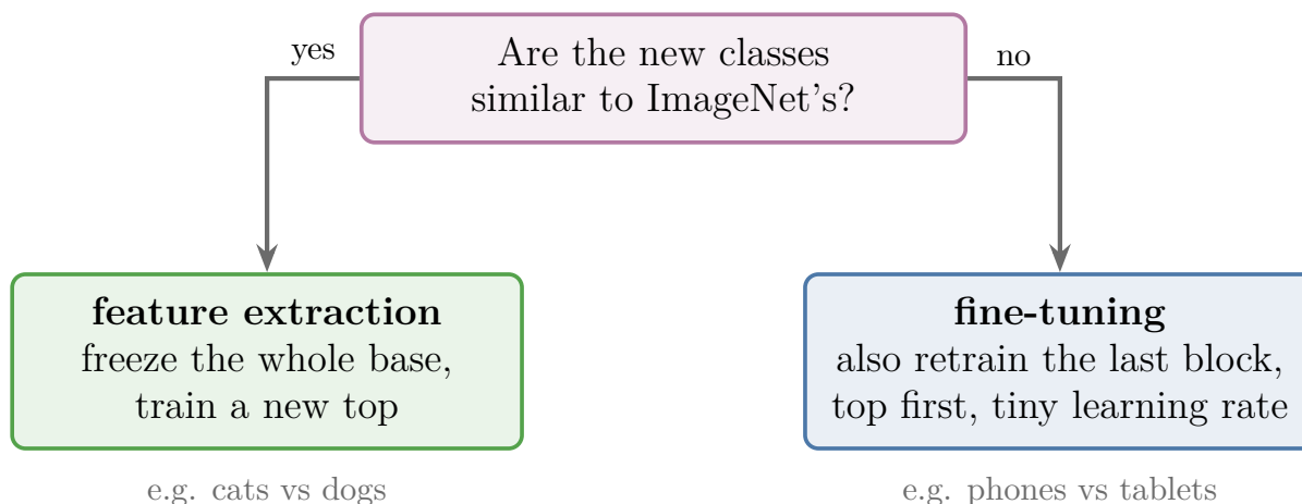
Figure 4: Choosing between the two forms of transfer, following sections 6.1 and 6.2.
