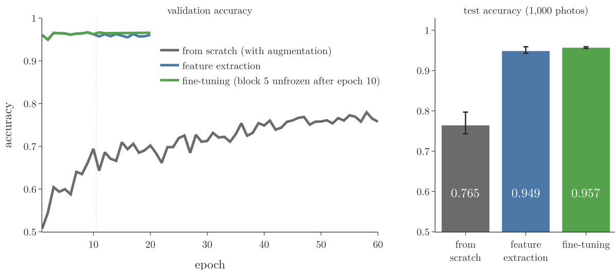
Figure 6: Validation accuracy per epoch (left; mean of 3 seeds) and test accuracy (right; bars: mean, whiskers: lowest and highest of 3 seeds). The dotted line marks where fine-tuning unfreezes block 5
