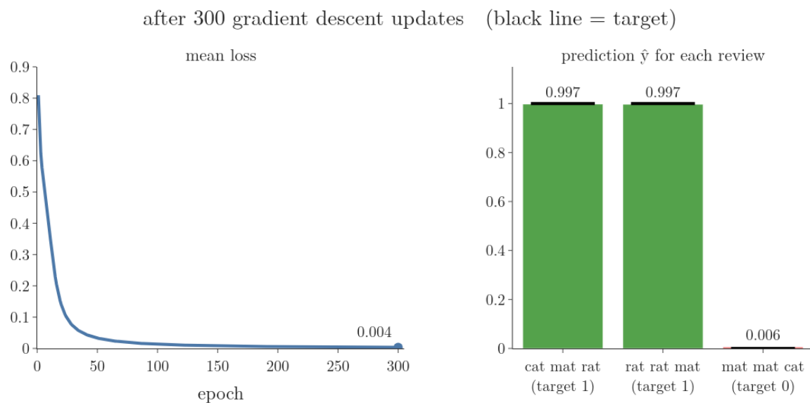
Figure 6: The training loop on the three toy reviews. Left: the mean loss per epoch. Right: the prediction for each review; the black line marks its target
