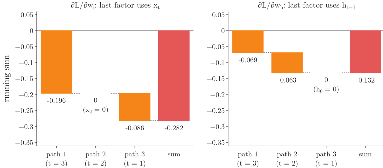
Figure 4: The gradient of a shared weight as a running sum of one term per time step, for w_i (left, this section) and w_h (right, section 7). Orange bars are the path terms; the red bar is the total
