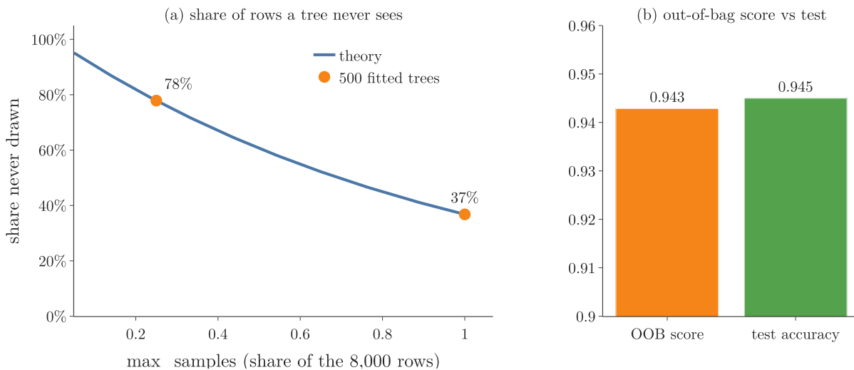
Figure 4: (a) Share of the 8,000 training observations a tree never draws, against max_samples : the theory curve (1 - 1/n) raised to the number of draws, and the mean over 500 fitted trees. (b) The out-of-bag score against the test accuracy
