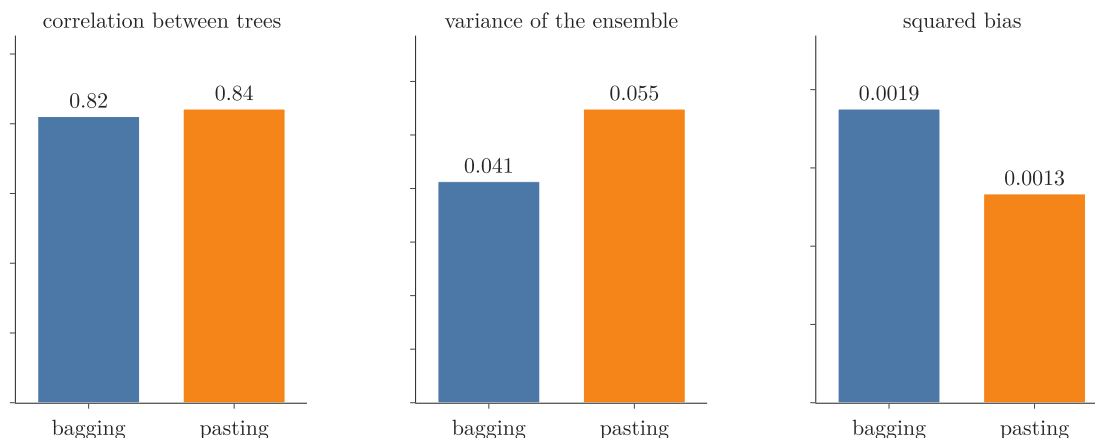
Figure 5: Bagging against pasting on 100 noisy sine datasets, changing only bootstrap : tree correlation, ensemble variance and squared bias
