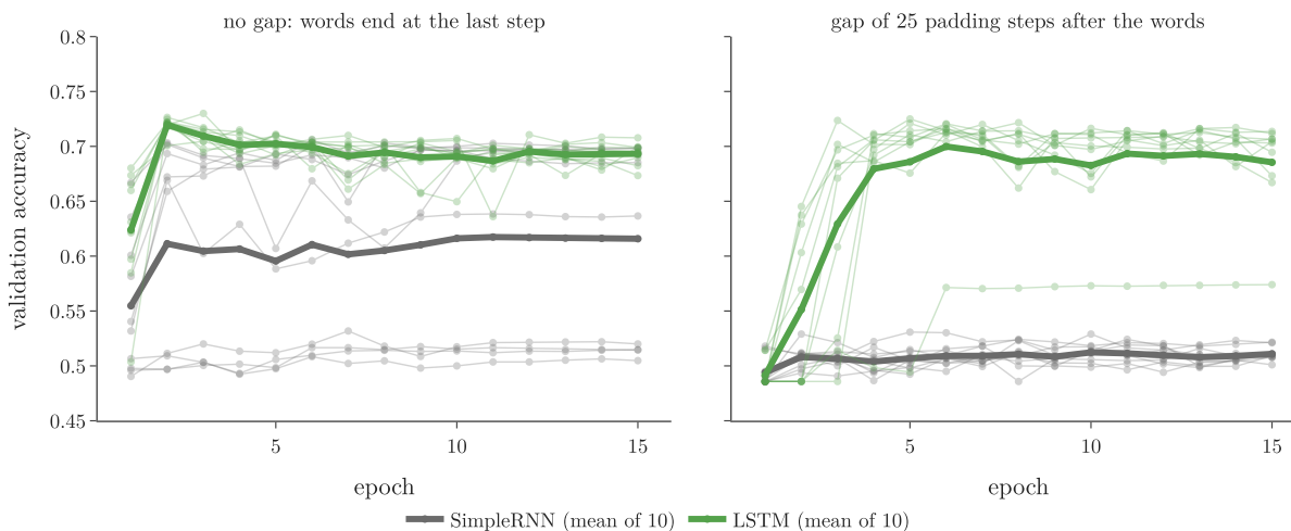
Figure 7: Validation accuracy of SimpleRNN (grey) and LSTM (green). Thin lines: 10 runs each; thick lines: their mean. The dotted line is 0.5. With 25 padding steps after the words, every SimpleRNN run stays near chance
