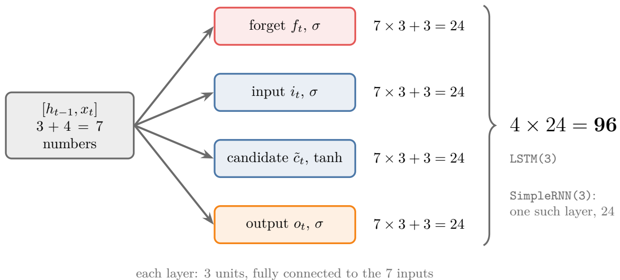
Figure 6: Where the 96 parameters of LSTM(3) on 4 input features come from: four layers, each fully connected from the 7 numbers of [h_{t-1}, x_t] to 3 units, so 7 \times 3 weights plus 3 biases each
