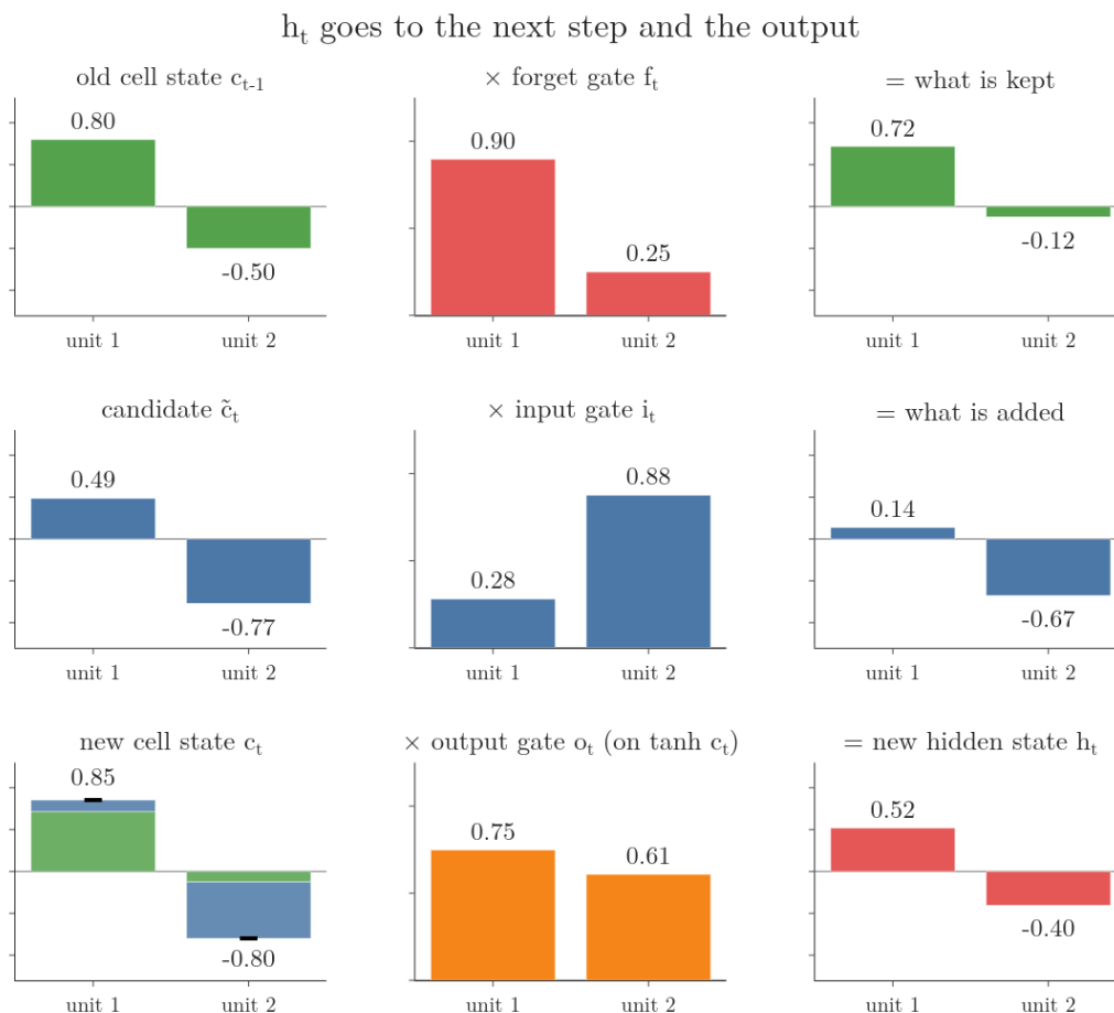
Figure 5: The time step above, one vector per frame. Each row is “value \times gate = result”: the forget gate scales the old cell state, the input gate scales the candidate, and the output gate scales \tanh(c_t) . The new cell state is drawn as what is kept (green) plus what is added (blue)
