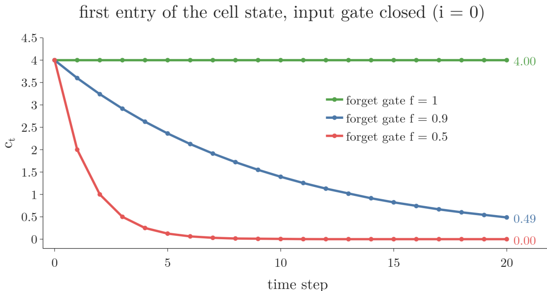
Figure 4: The first entry of the cell state [4, 5, 6] over 20 time steps with the input gate closed, for three forget-gate values. Only f = 1 carries the value unchanged
