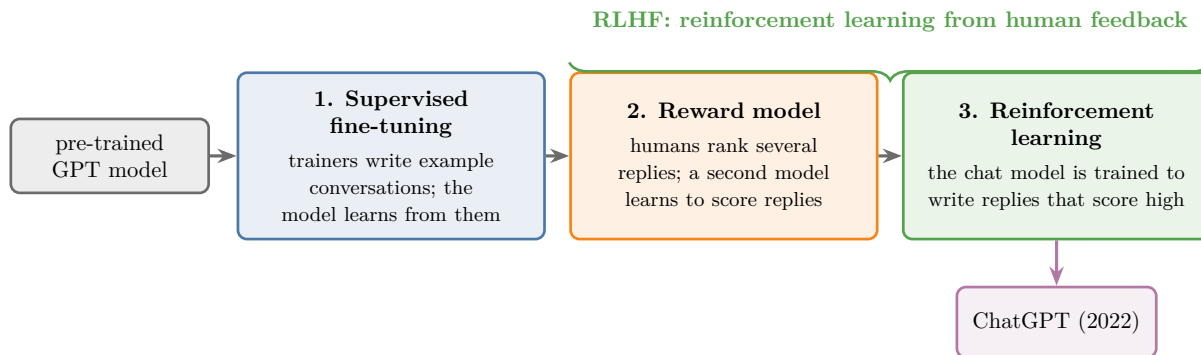
Figure 8: The three training steps of ChatGPT, after pre-training. Steps 2 and 3 form reinforcement learning from human feedback (RLHF)
