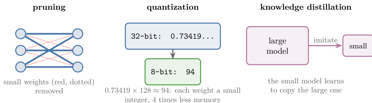
Figure 8: Three ways to make a model smaller. Pruning removes the connections with small weights; quantization stores each weight as an 8-bit integer instead of a 32-bit number; knowledge distillation trains a small model to imitate a large one
