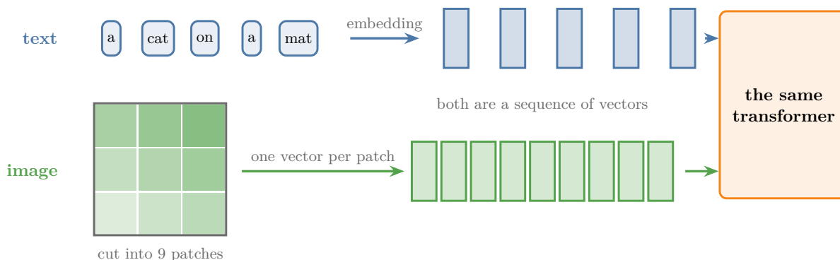
Figure 5: Text and an image as sequences of vectors. Each word becomes one vector through an embedding; the image is cut into patches, and each patch becomes one vector. The same transformer can then read either sequence
