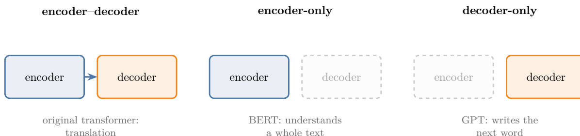
Figure 7: The three layouts of a transformer: the full encoder–decoder of the original paper, the encoder alone (BERT) and the decoder alone (GPT)
