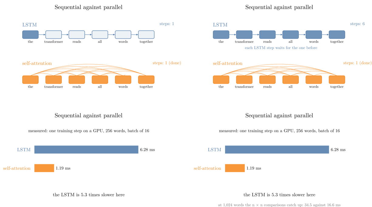
Figure 3: Sequential against parallel. Top: the LSTM reads one word per step, each step waiting for the one before. Bottom: self-attention computes every position in one step, every word looking at every word. Then the measured time of one training step at 256 words
