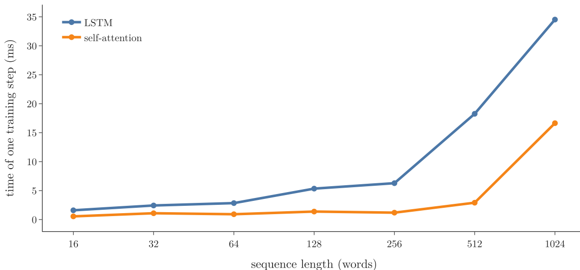
Figure 4: Time of one training step against sequence length (log scale). The LSTM’s time grows from the start; self-attention stays flat up to 256 words
