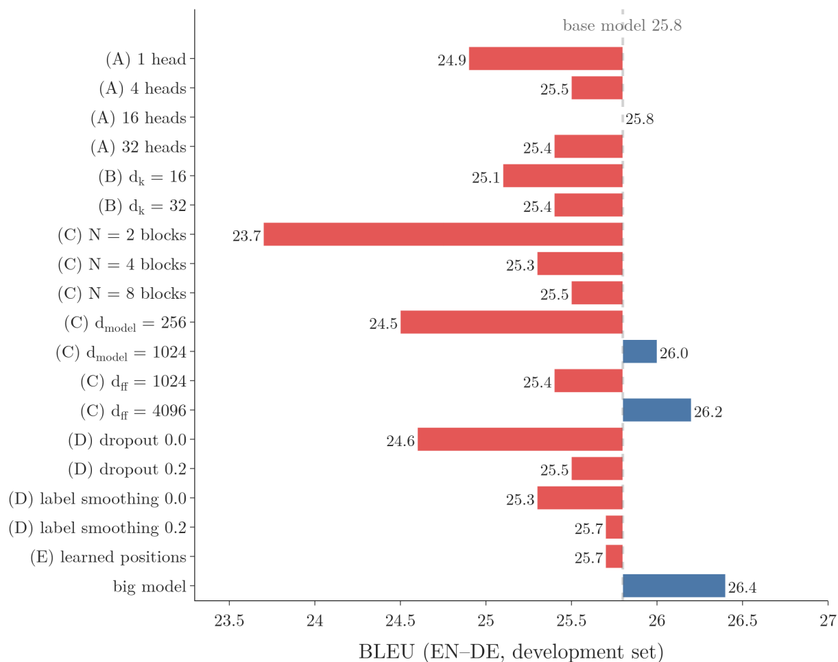
Figure 10: Table 3 as bars around the base model’s 25.8 BLEU: blue rows beat the base model, red rows fall below it
