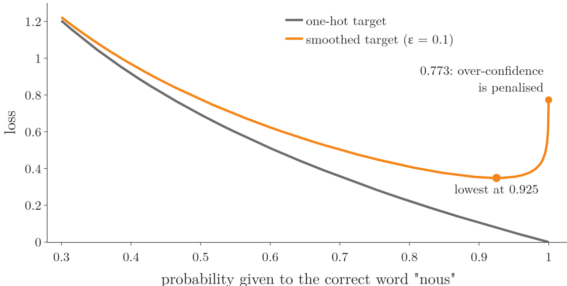
Figure 8: The two losses as the probability of the correct word “nous” grows from 0.30 to 0.9999, with the rest shared evenly. The one-hot loss keeps falling towards certainty; the smoothed loss is lowest at 0.925 and rises again
