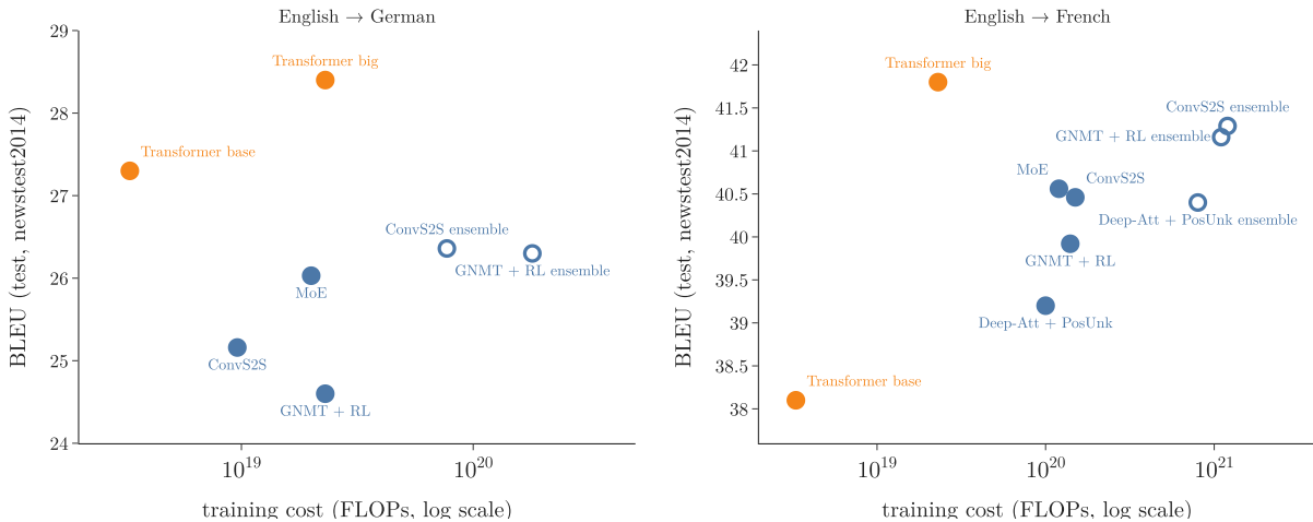
Figure 9: Table 2 of the paper: BLEU against training cost. Orange: the transformer. Hollow circles: ensembles. ByteNet has no listed cost and is left out
