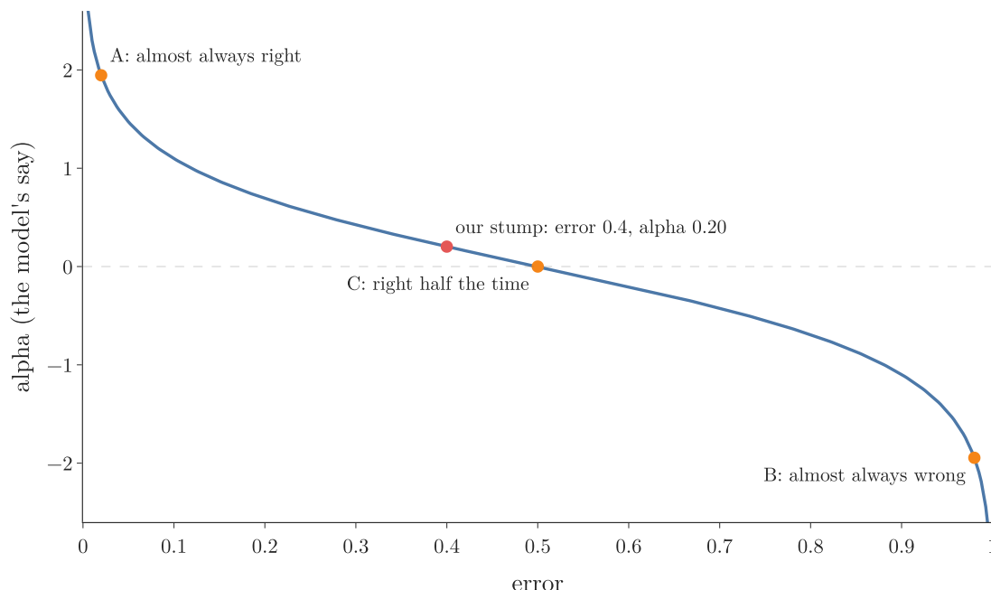
Figure 3: Alpha against the error: model A (error near 0) gets a large positive say, model C (error 0.5) none, model B (error near 1) a large negative say
