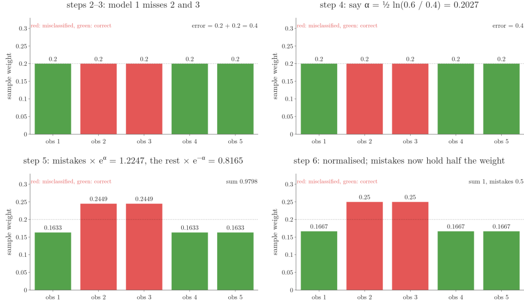
Figure 4: The 5 sample weights through one stage of the worked example: equal at 0.2, observations 2 and 3 misclassified (error 0.4, alpha 0.2027), multiplied by e^\alpha or e^{-\alpha} , then normalised
