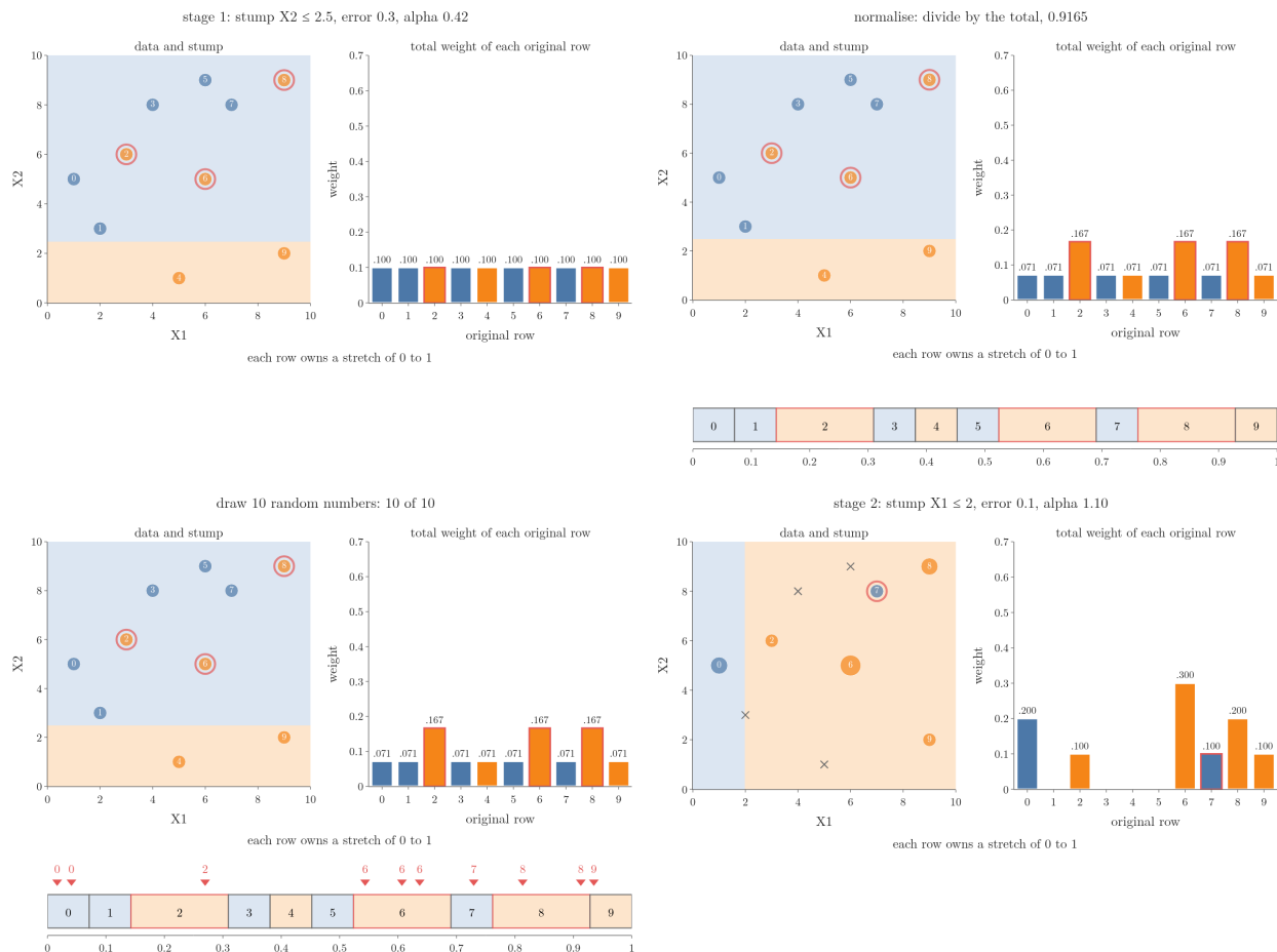
Figure 5: The AdaBoost loop on the toy data: the stump and its mistakes (red rings), the weight of each original row (a row drawn twice counts 0.2), and the stretch of 0 to 1 each row owns, with the ten random draws as darts
