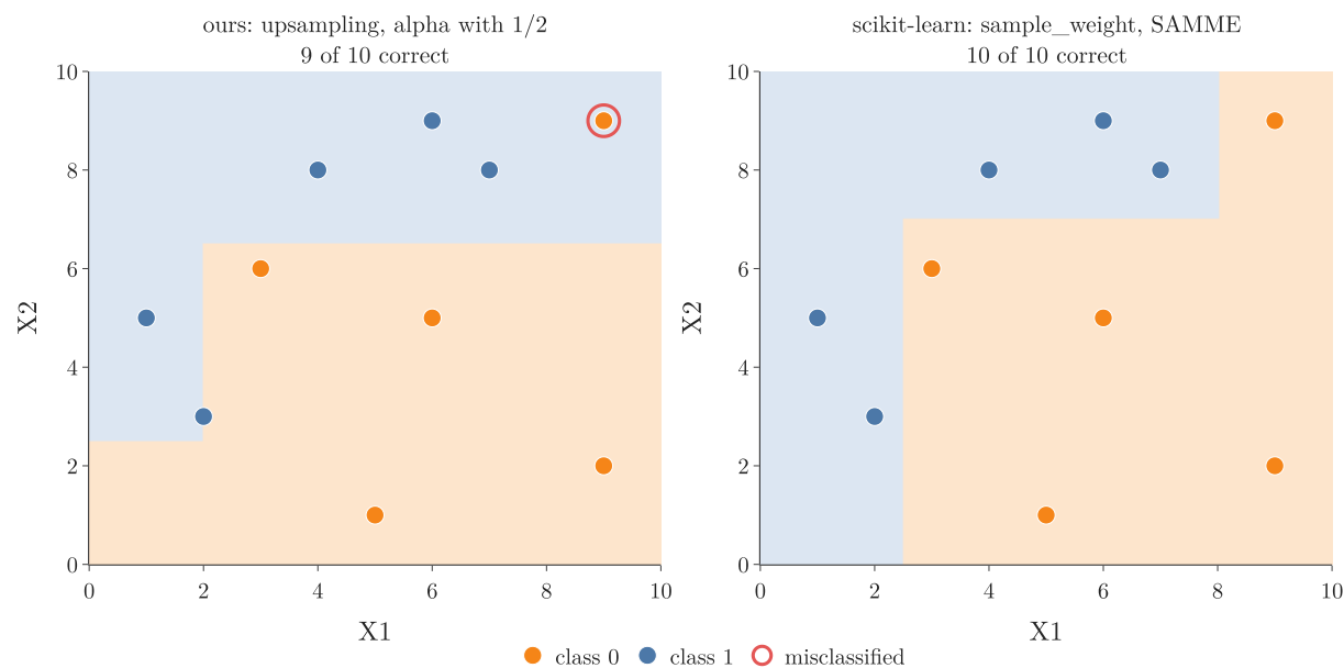
Figure 8: Decision regions of our three upsampled stumps (left, 9 of 10 correct, observation 8 missed) and scikit-learn's three weighted SAMME stumps (right, 10 of 10 correct)
