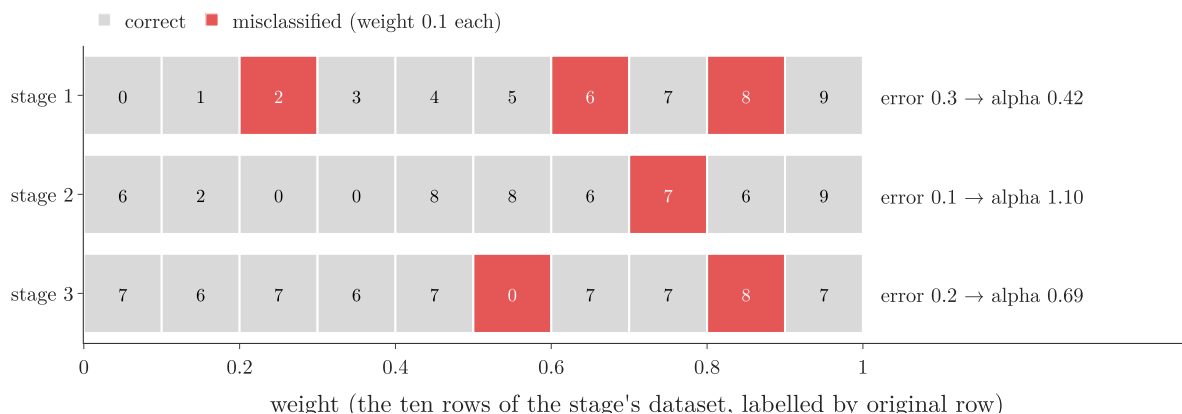
Figure 2: The error of each stage is the total weight of its mistakes (red); each block is one row of that stage's dataset, labelled by its original row. Stage 1 covers 0.3 of the bar, stage 2 covers 0.1, stage 3 covers 0.2
