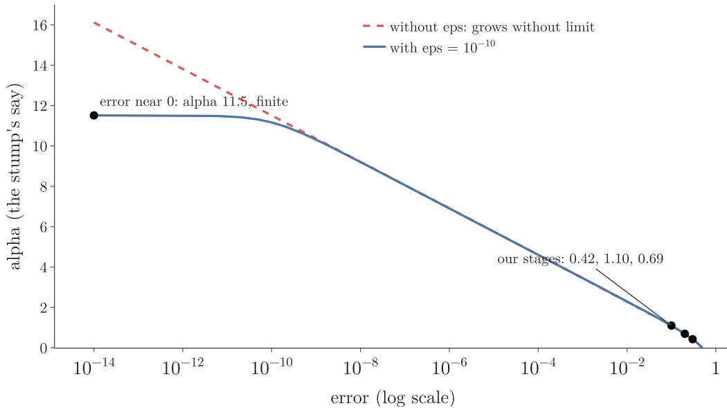
Figure 6: Alpha against the error on a log scale. Without eps (dashed) alpha grows without limit as the error falls to 0; with \text{eps} = 10^{-10} it levels off at 11.5. Our three stages sit at the far right
