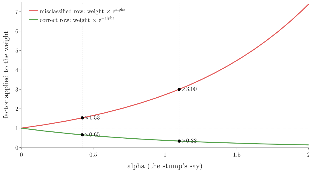
Figure 4: The factors e^\alpha (mistakes) and e^{-\alpha} (correct observations) against alpha, marked at our stage 1 and stage 2 alphas
