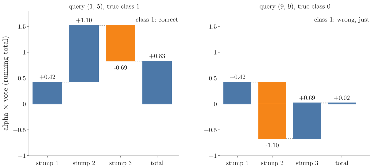
Figure 7: The weighted vote built up stump by stump, alpha times the stump's +1 or -1. Query (1, 5) ends at +0.83, class 1, correct; query (9, 9) ends at +0.02, class 1, wrong
