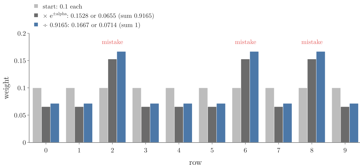
Figure 3: Stage 1 weights per row: the start (0.1), after the exponential update (0.1528 or 0.0655, total 0.9165), and after dividing by 0.9165 (0.1667 or 0.0714, total 1)
