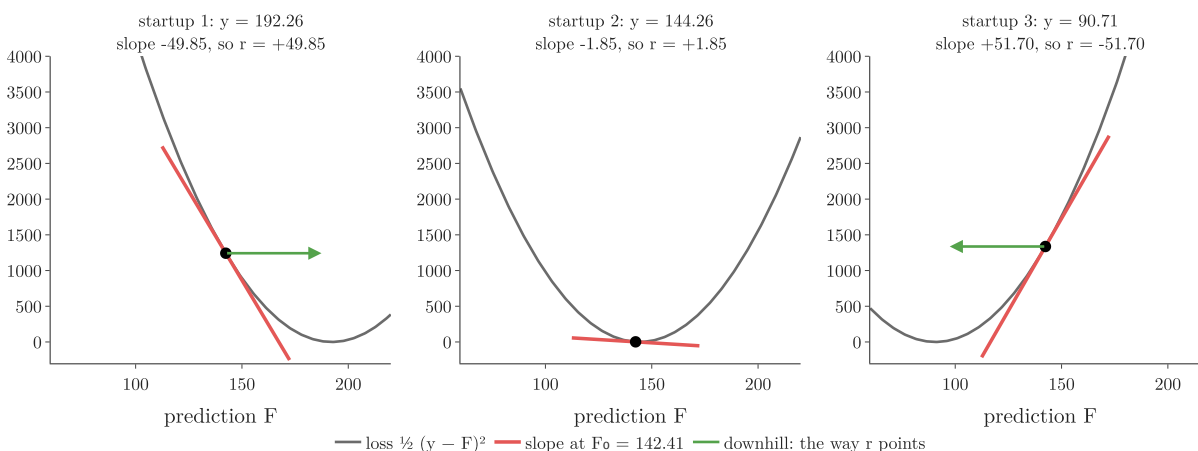
Figure 4: Each startup’s loss \frac{1}{2}(y - F)^2 against the prediction F . The red line is the slope at F_0 = 142.41 ; the pseudo-residual is minus that slope, and the green arrow is the downhill direction
