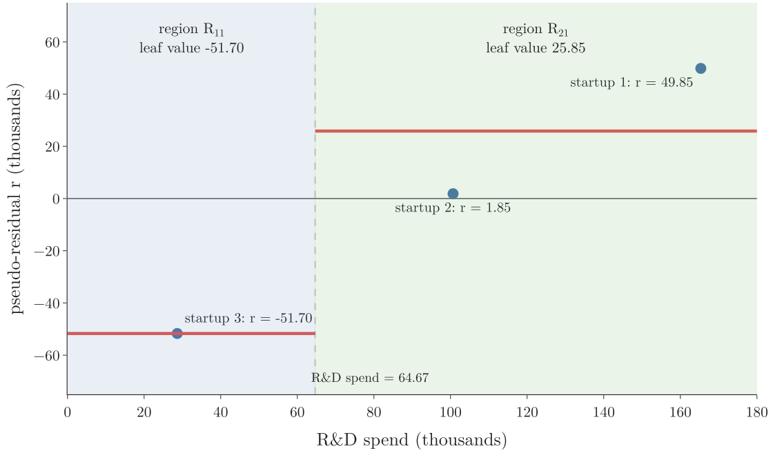
Figure 5: The first tree on the pseudo-residuals: one split on R&D spend makes two terminal regions, each with its leaf value
