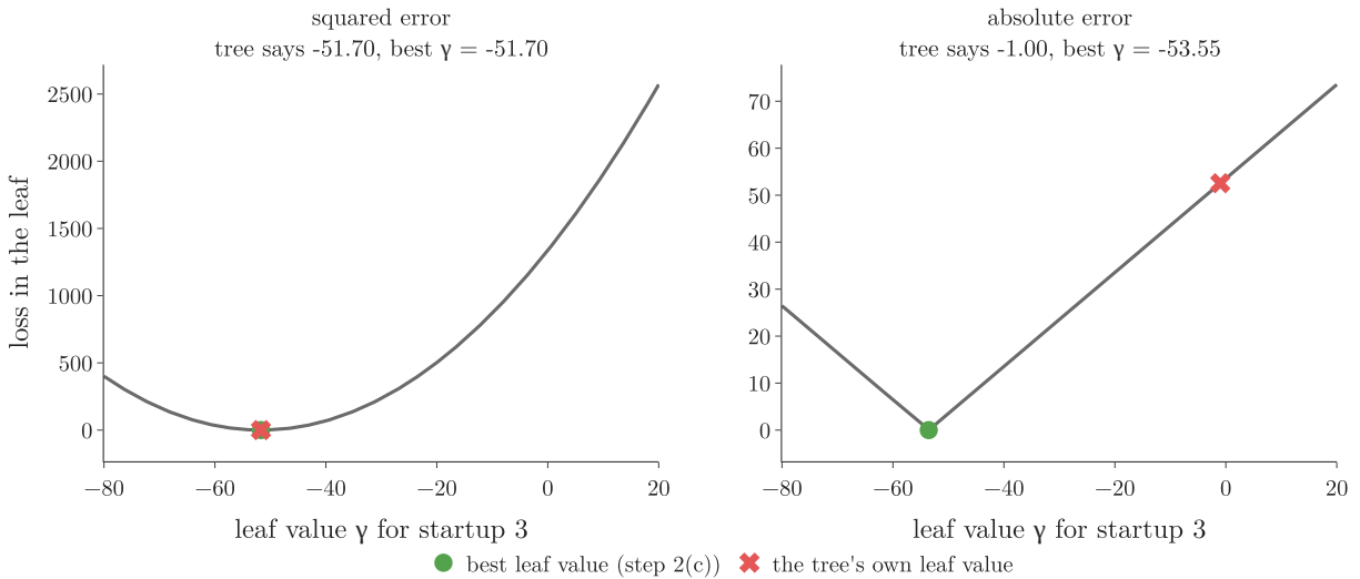
Figure 6: Loss in region R_{11} against the leaf value. Squared error (left): the tree's own value, -51.70 , is the minimum. Absolute error (right): the tree's own value, -1 , is far from the minimum at -53.55
