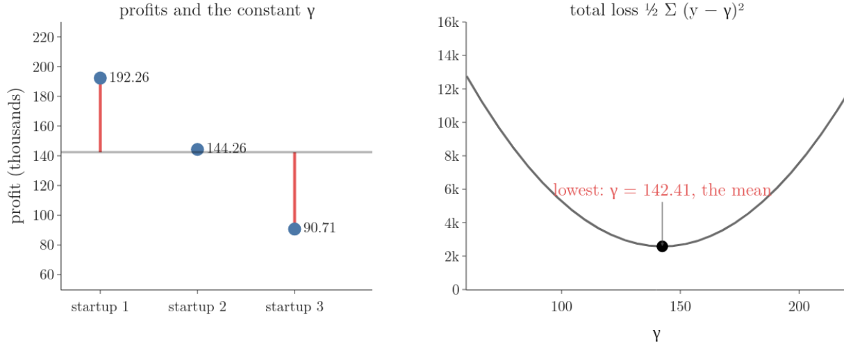
Figure 3: Step 1 on the three startups: the constant \gamma (black line) and the gaps to each profit (left), and the total loss against \gamma (right); the lowest loss is at the mean, 142.41
