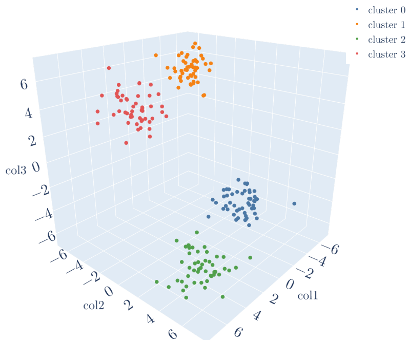
Figure 5: k-means with k = 4 on 200 points with three features
