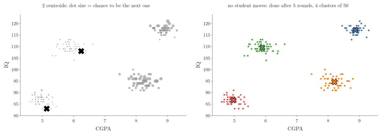
Figure 3: k-means on the 200 students, k = 4 , unscaled. First a k-means++ start (the plain version; scikit-learn runs a greedy variant): dot size is a student’s chance to become the next centroid. Then assign and update rounds until no student moves: four clusters of 50
