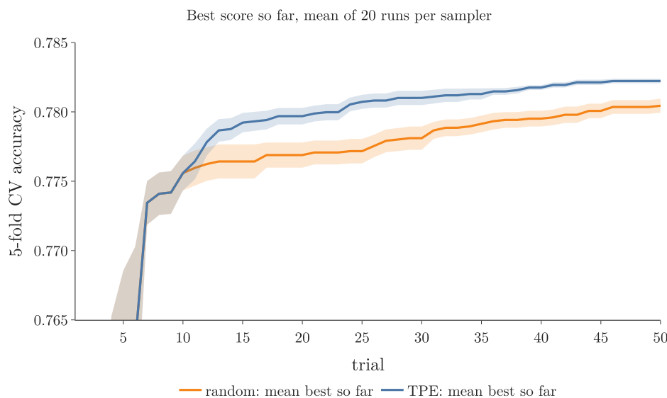
Figure 5: Best 5-fold CV accuracy so far, averaged over 20 runs of each sampler on the SVM search; the bands are \pm one standard error
