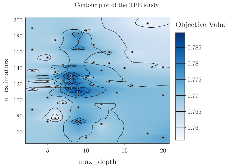
Figure 8: Contour plot of the TPE study: max_depth against n_estimators , darker is a higher score; dots are trials
