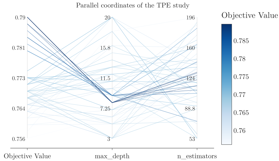
Figure 7: Parallel coordinates of the TPE study: each line is a trial, darker is a higher score
