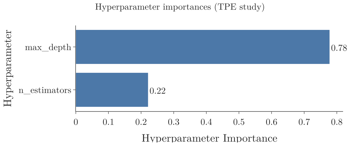
Figure 9: Hyperparameter importances of the TPE study
