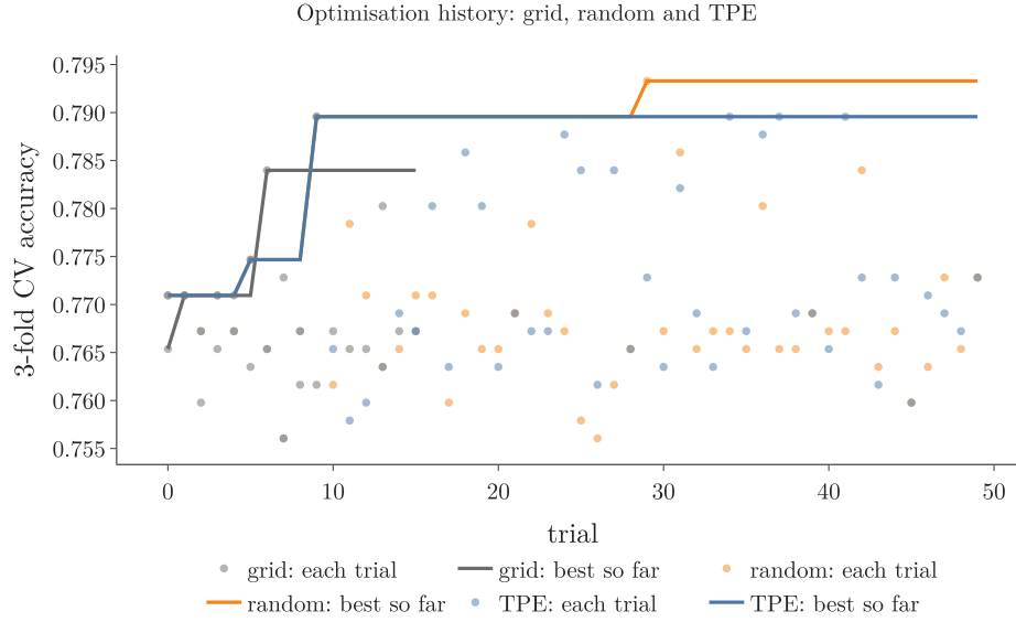
Figure 6: Optimisation history of the three studies: each trial (dots) and the best so far (lines)
