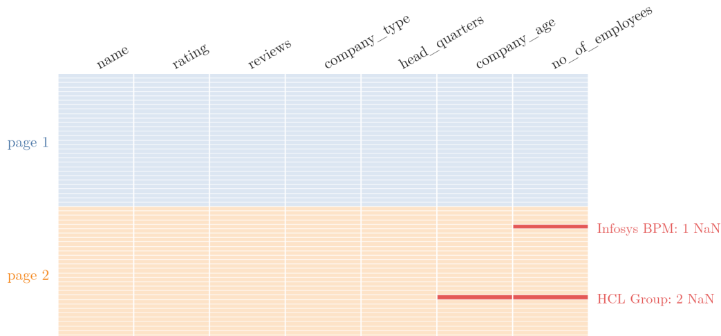
Figure 8: The 60 x 7 table from the two saved pages; the 3 NaN cells are red
