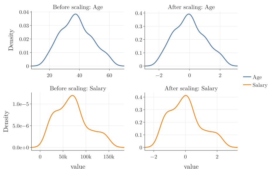
Figure 7: Each column's distribution before and after: the shape stays, the numbers change
