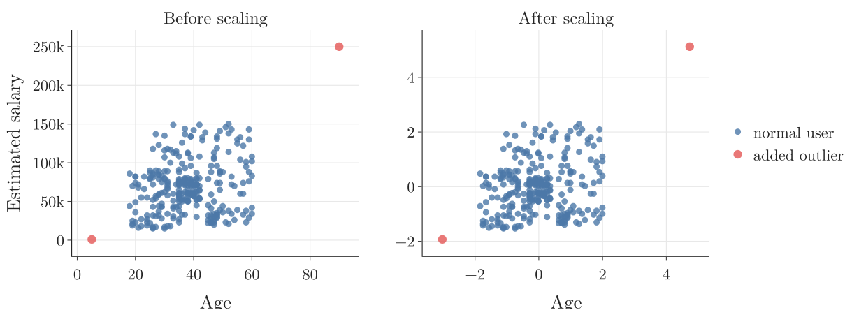
Figure 9: Two added outliers (red) before and after standardization
