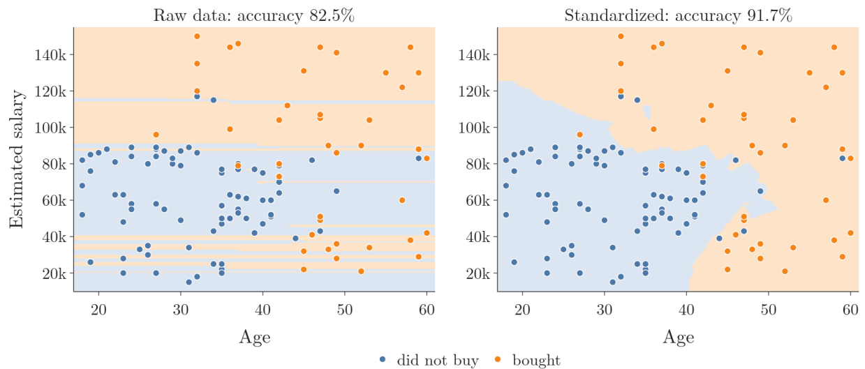
Figure 8: Where KNN (5 neighbours) predicts “bought” (orange) and “did not buy” (blue), trained on raw and on standardized data; dots are the 120 test users
