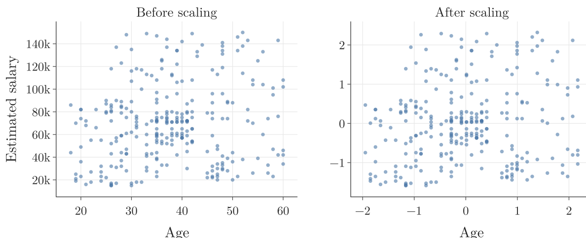
Figure 5: The training data before and after standardization
