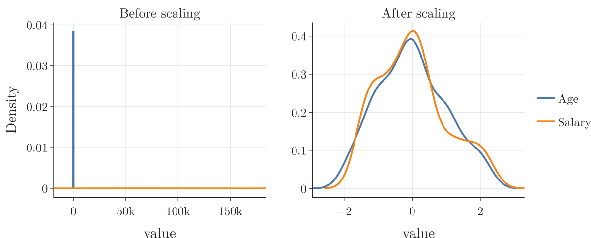
Figure 6: Density curves of age (blue) and salary (orange), before and after standardization
