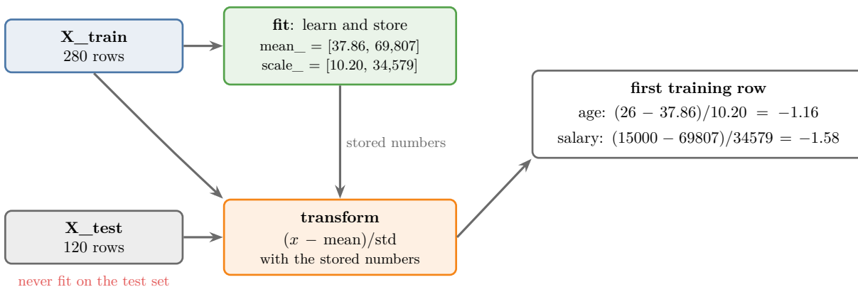
Figure 4: fit learns the mean and standard deviation from the 280 training rows; transform applies them to both sets, here to the first training row
