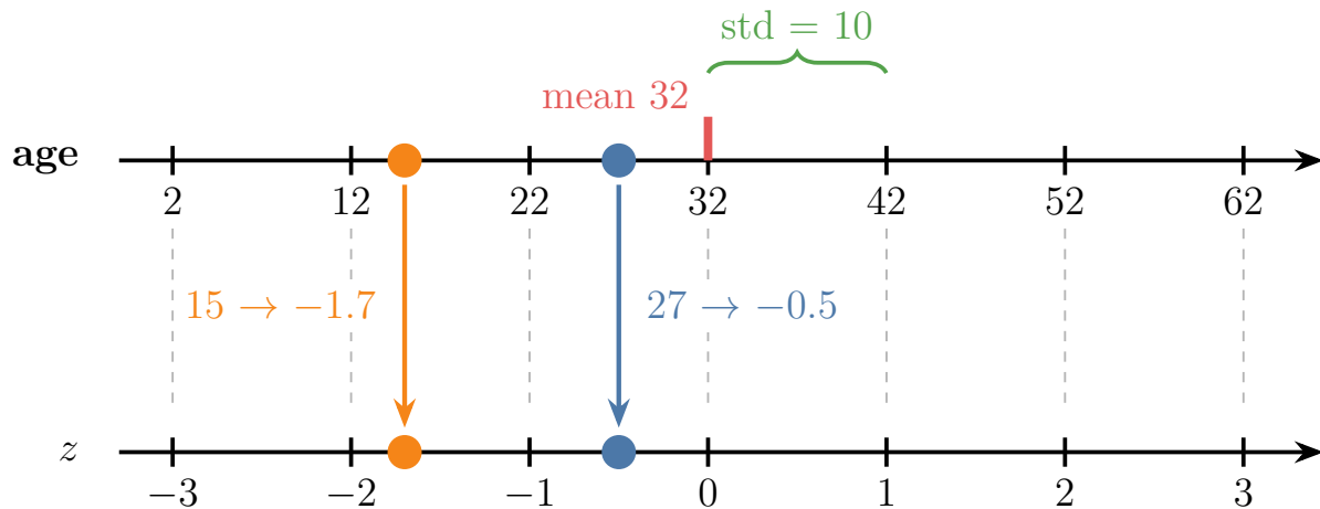
Figure 2: The ages 27 and 15 on the age line (mean 32, std 10) and the same two customers on the z line
